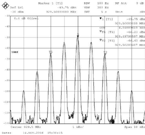
929.5 MHz 4K00F3E input (left) and output (right), level above AGC threshold
