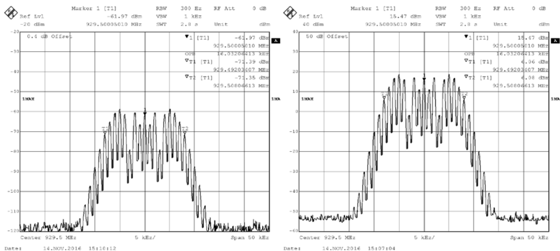
929.5 MHz 16K0F3E input (left) and output (right), level below AGC threshold
