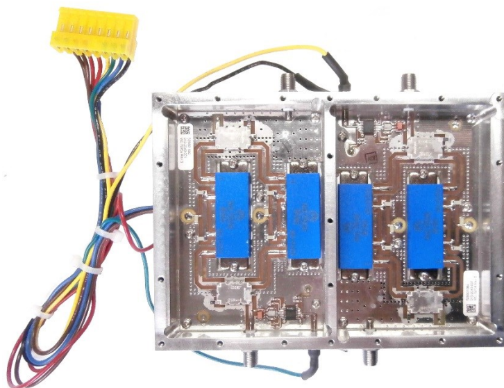
010-2043-001 COMP SIDE
