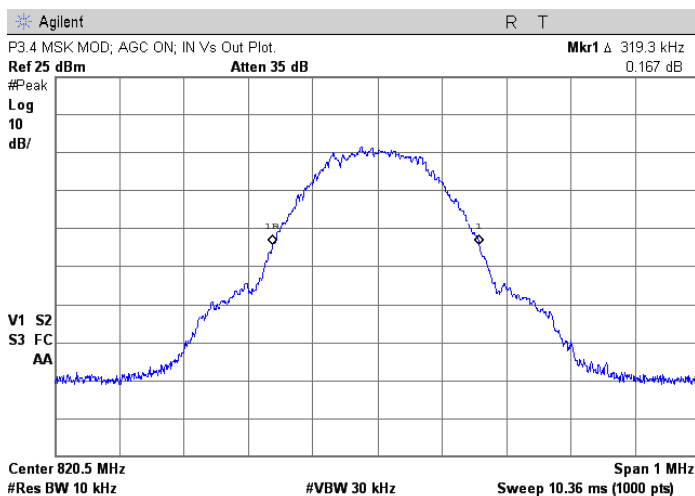
Amp output with AGC; 820.5 MHz, MSK
