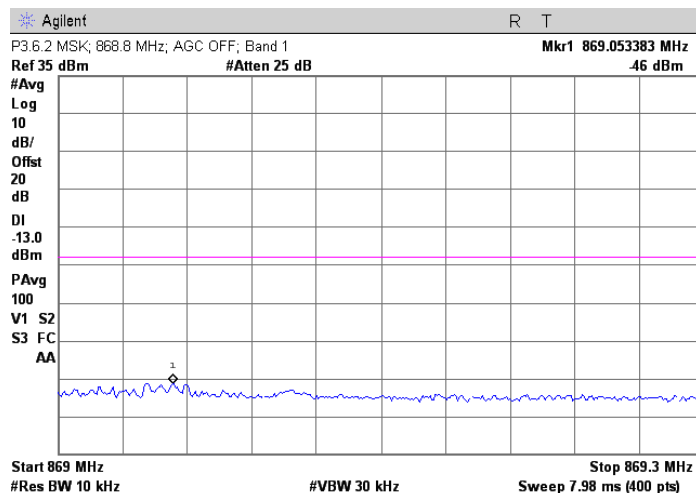
MSK; 868.8 MHz Injected Signal; AGC off
