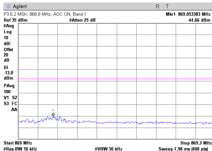
MSK; 868.8 MHz Injected Signal; AGC on
