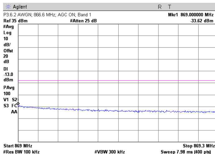
AWGN; 866.6 MHz Injected Signal; AGC on
