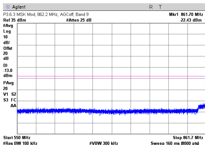
MSK ; 862.2 MHz Injected Signal
