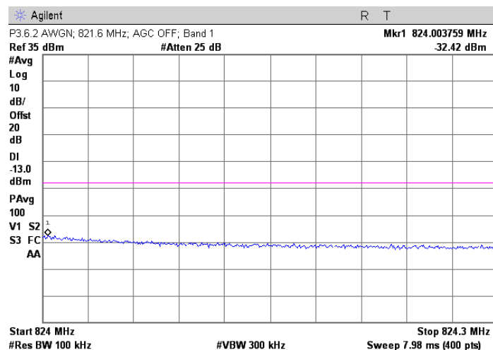
AWGN; 821.6 MHz Injected Signal; AGC off
