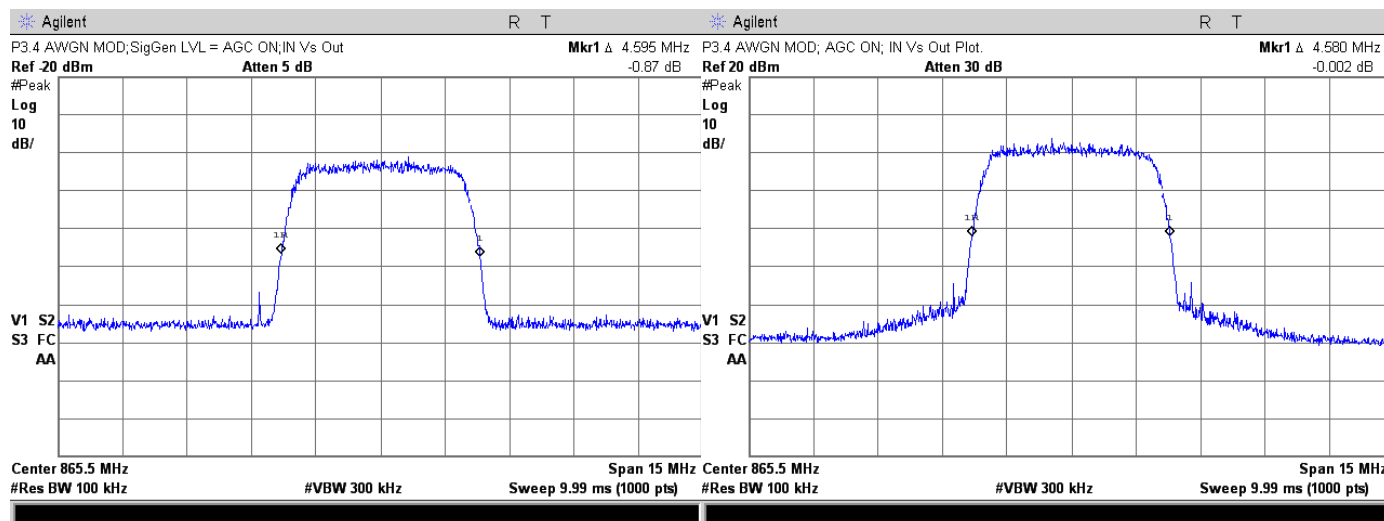
Generator output for AGC On ; 865.5 MHz, AWGN
