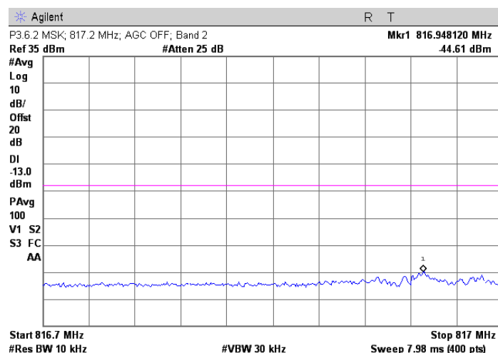
MSK; 817.2 MHz Injected Signal; AGC off
