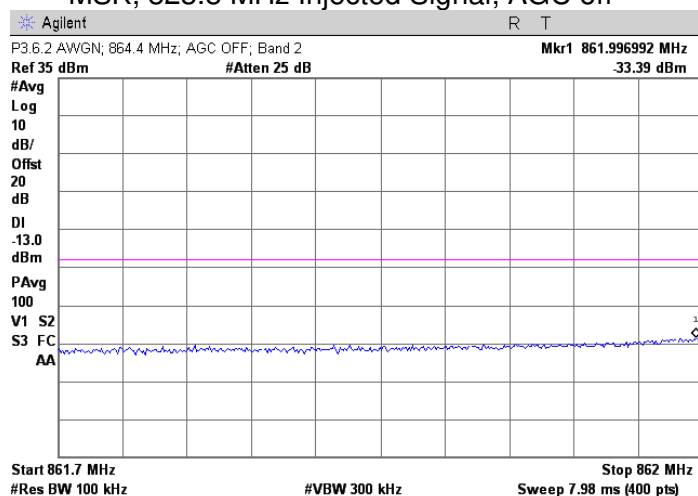
AWGN; 864.4 MHz Injected Signal; AGC off
