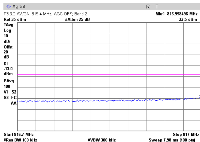
AWGN; 819.4 MHz Injected Signal; AGC off
