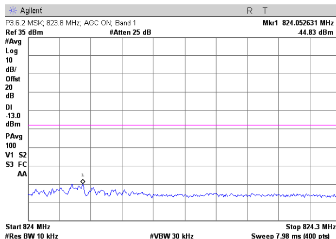
MSK; 823.8 MHz Injected Signal; AGC on
