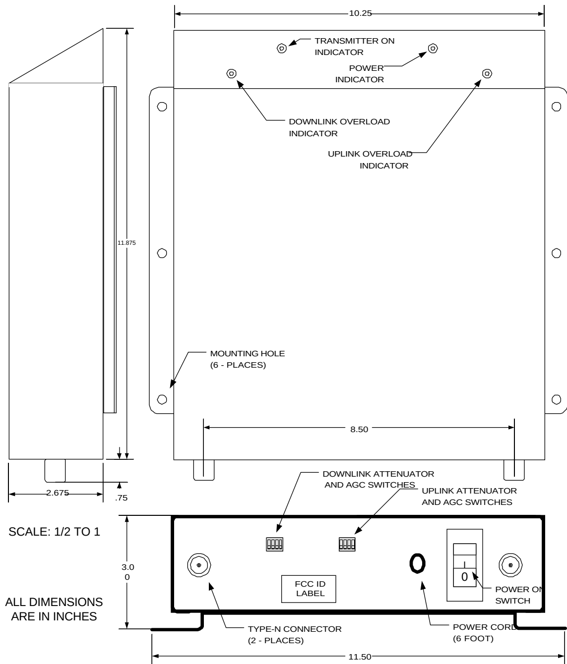
FIGURE 2.2 Model 310 Mechanical Outline Drawing
