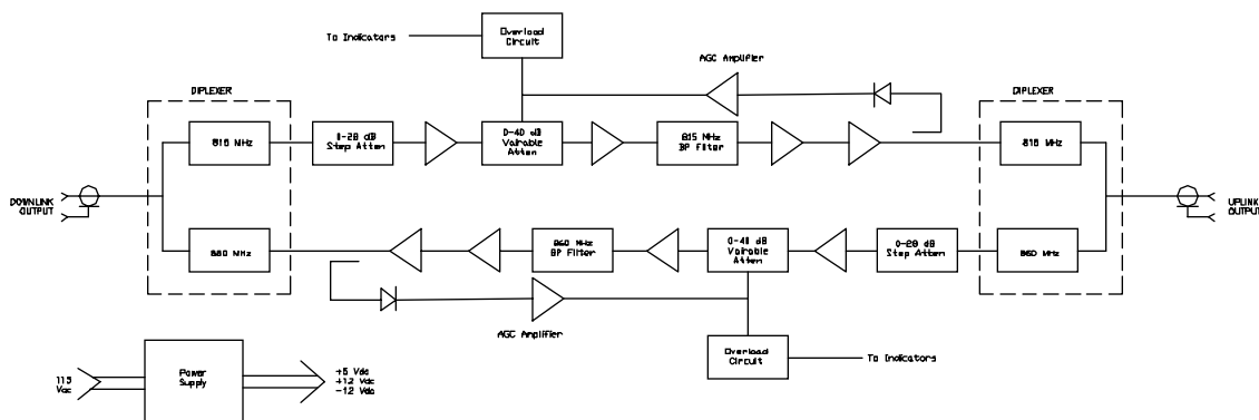
FIGURE 2.1 Functional Block Diagram
