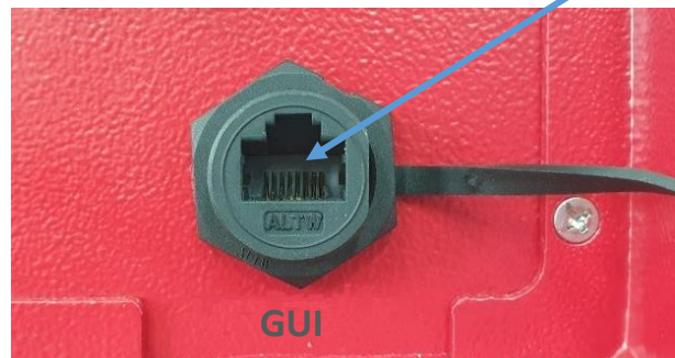
Figure 5-2B: Ethernet Connectors
