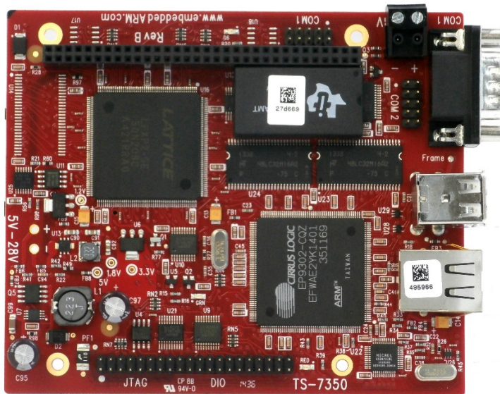
Single Board Computer Comp Side
