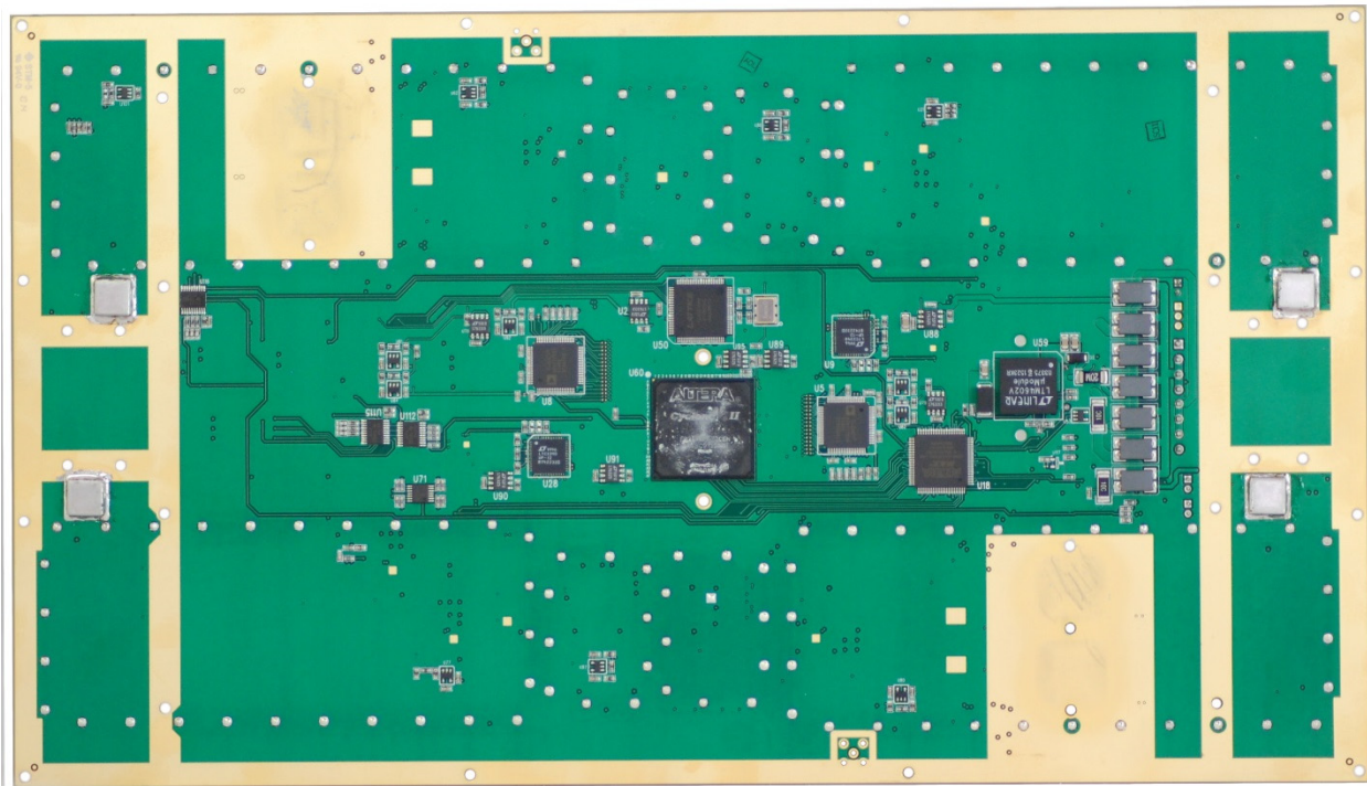
R010-2114-003 Non-Comp Side
