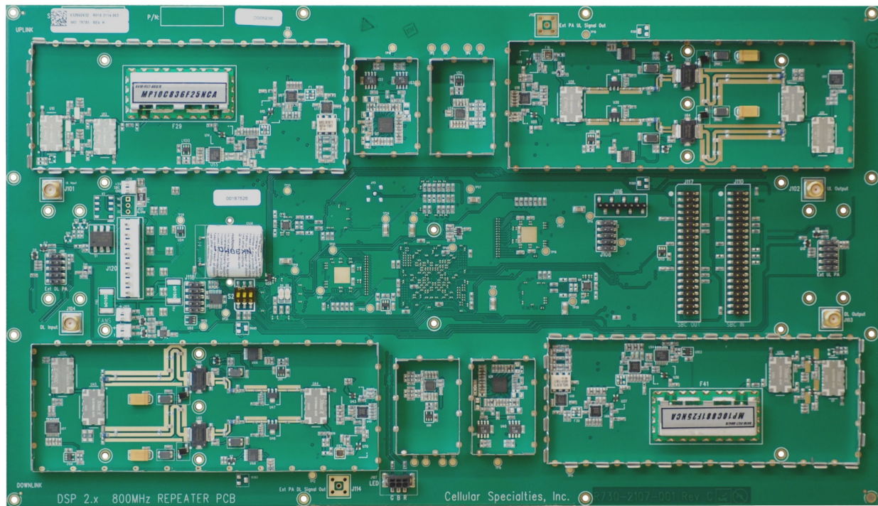
R010-2114-003 Comp Side
