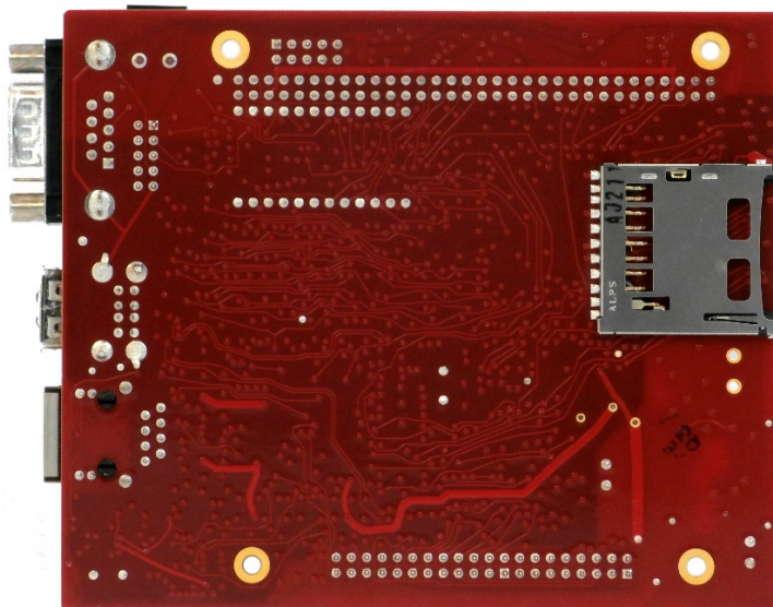
Single Board Computer Non-Comp Side
