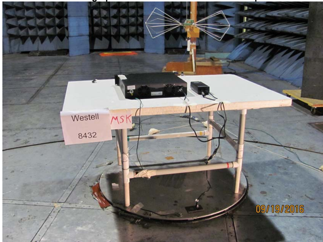
Photograph of Radiated Emissions Test Setup
