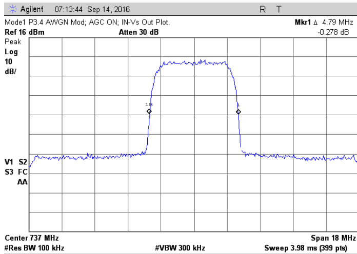
Amp output with AGC; 737 MHz, AWGN
