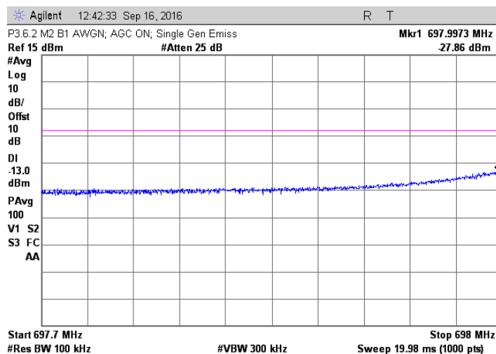
AWGN; 700.5 MHz Injected Signal; AGC on
