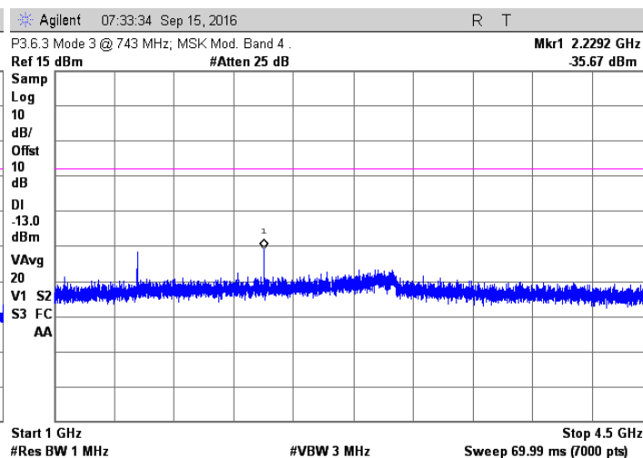
MSK; 743 MHz Injected Signal
