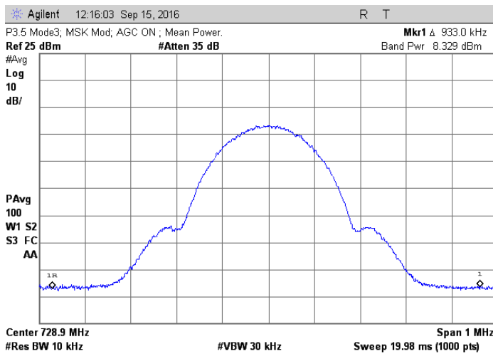
728.9 MHz MSK; AGC On
