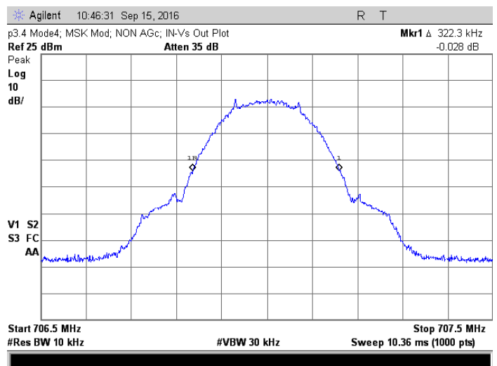
Amp output, no AGC; 707 MHz, MSK
