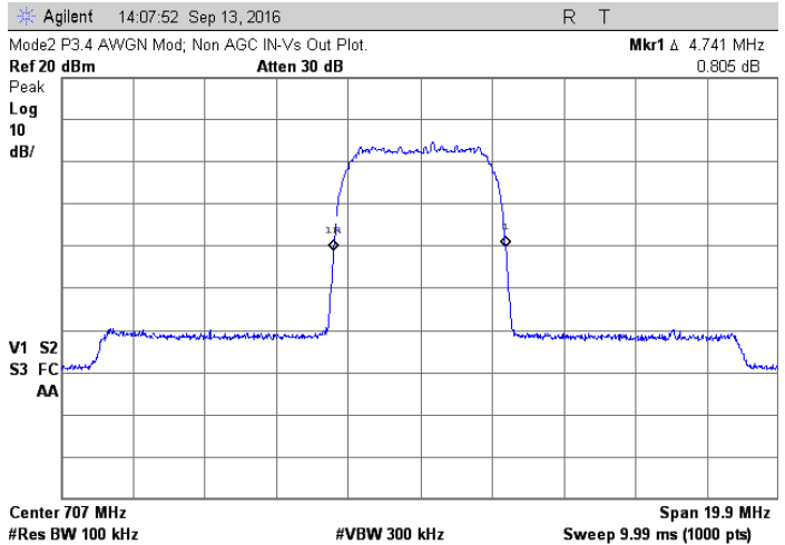
Amp output, no AGC; 707 MHz, AWGN
