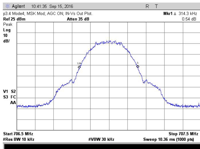
Amp output with AGC; 707 MHz, MSK
