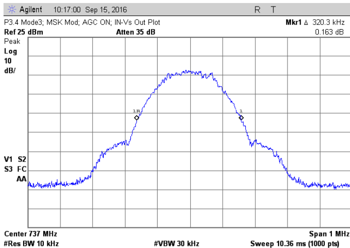
Amp output with AGC; 737 MHz, MSK
