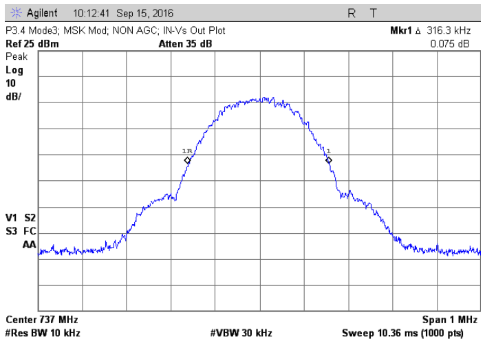
Amp output, no AGC; 737 MHz, MSK
