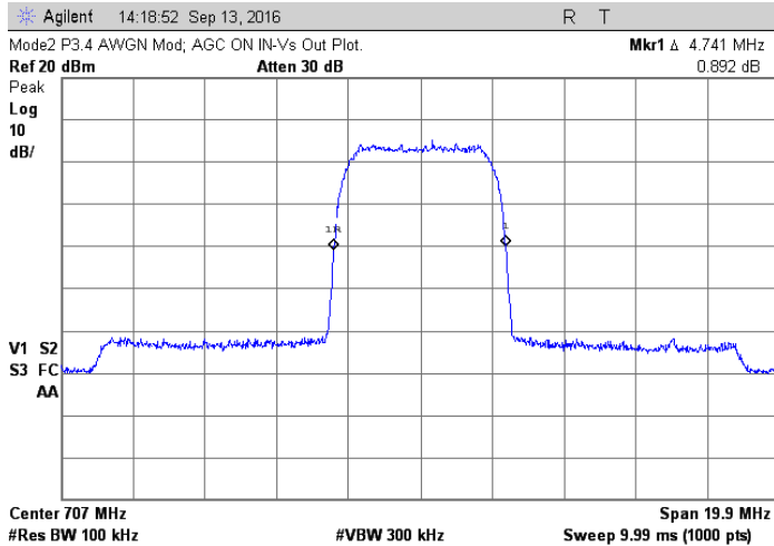
Amp output with AGC; 707 MHz, AWGN
