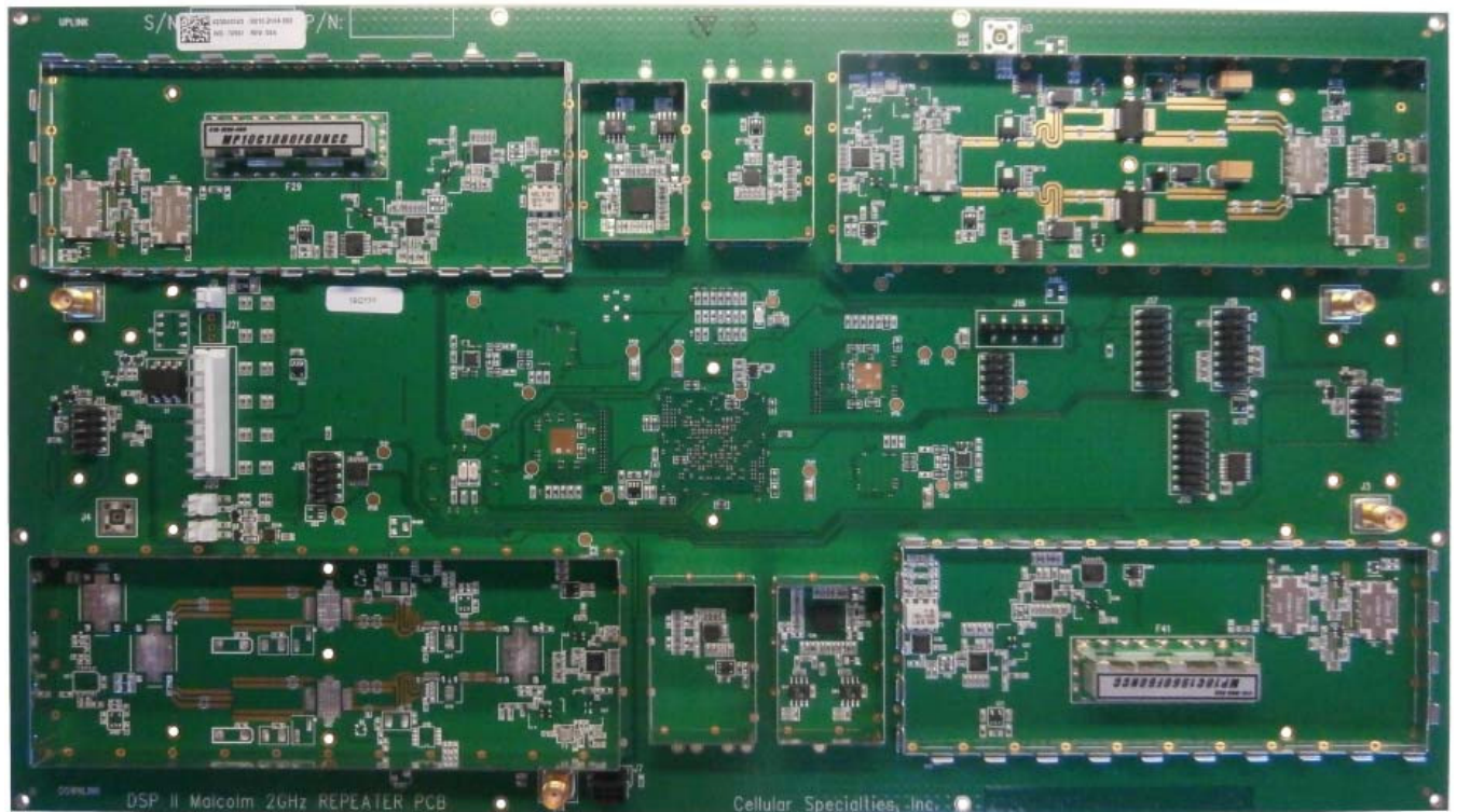
Figure 2. Repeater Boards
