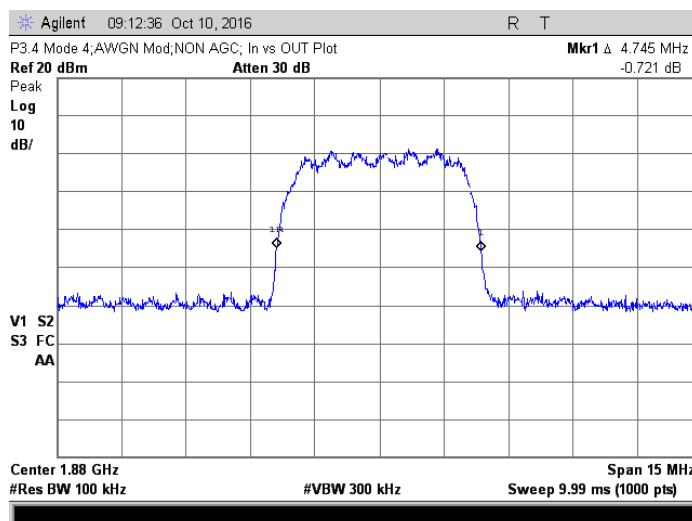
Amp output, no AGC; 1.88 GHz, AWGN
