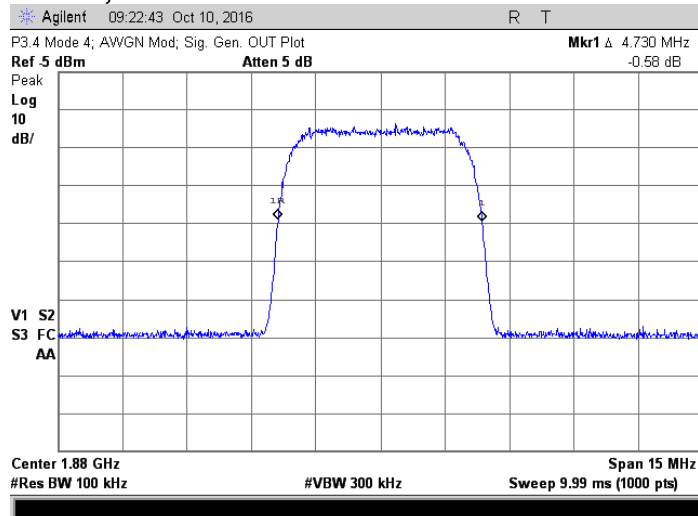
Generator output; 1.88 GHz, AWGN
