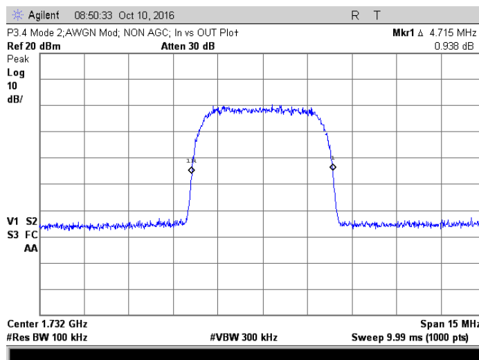
Amp output, no AGC; 1.732 GHz, AWGN
