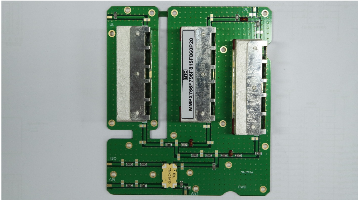
DL MUX PCB
