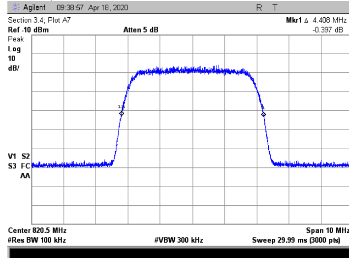
Generator output; 820.5 MHz, AWGN
