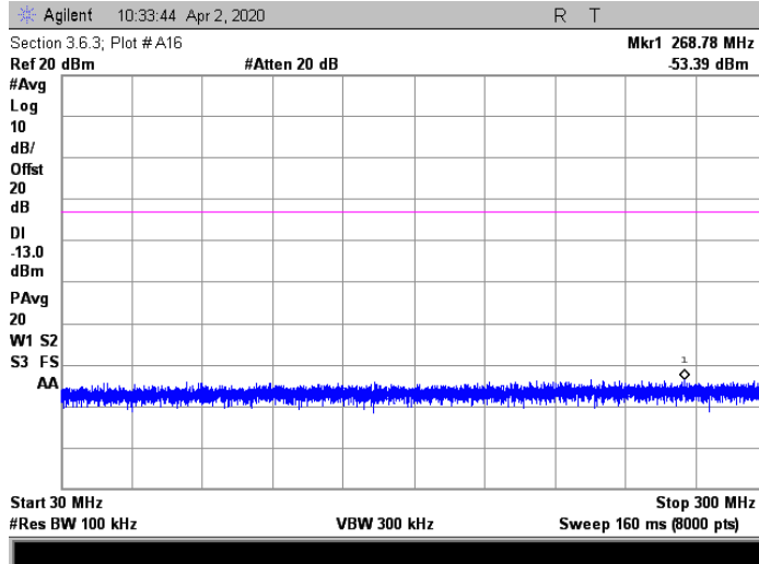
AWGN; 864.4 MHz Injected Signal
