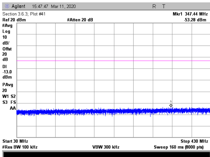
MSK ; 823.6 MHz Injected Signal
