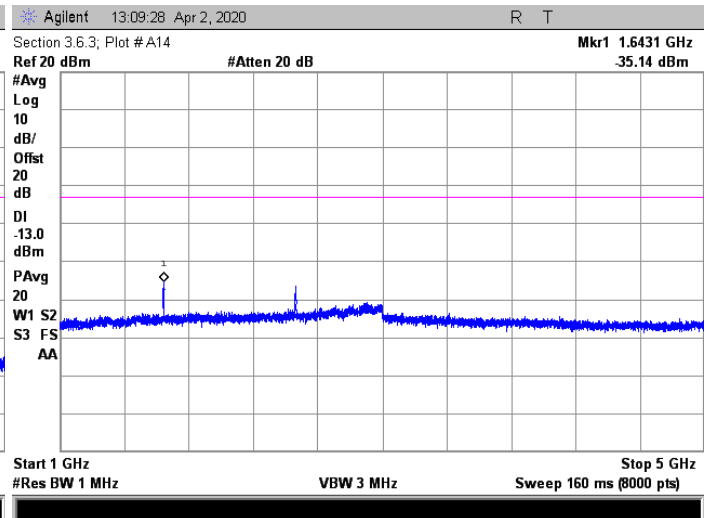
AWGN; 821.6 MHz Injected Signal
