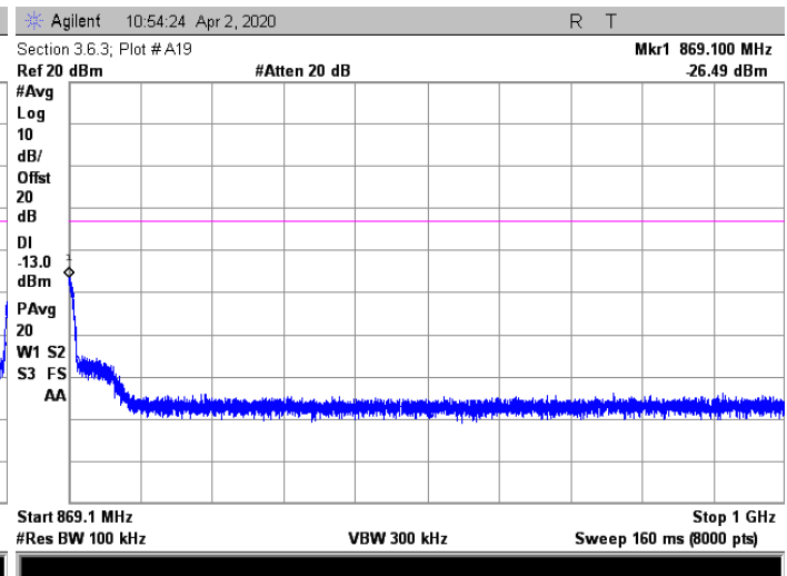
AWGN; 864.4 MHz Injected Signal
