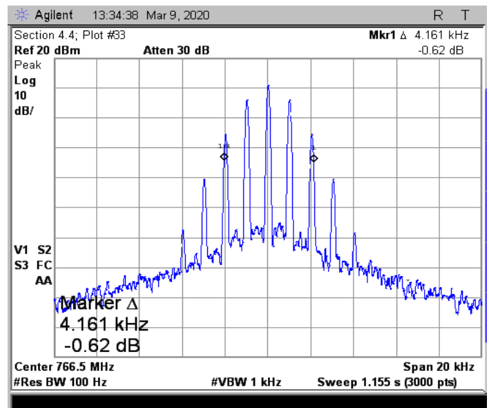
AMP Output: Level above AGC; FM 4K
