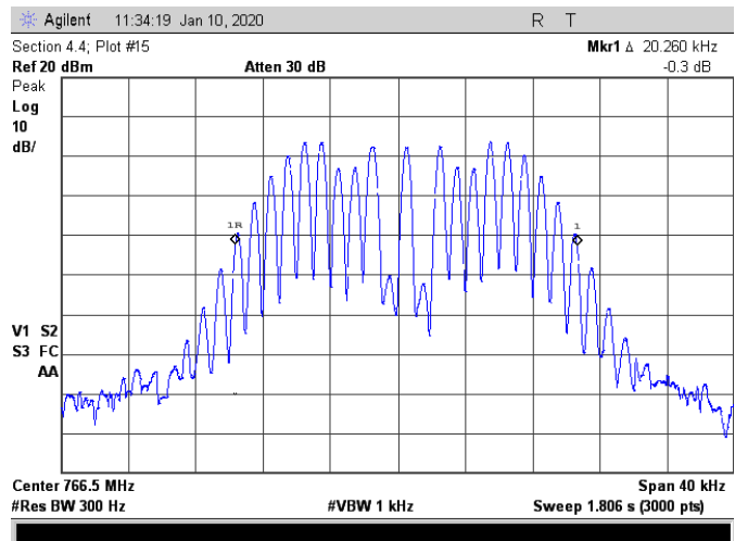
AMP Output: Level Above AGC; FM 16K
