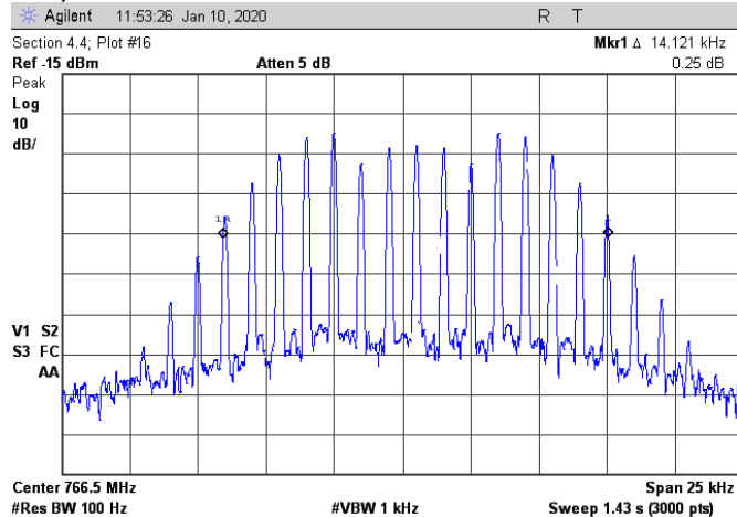
Input Signal to Amp; FM 11K
