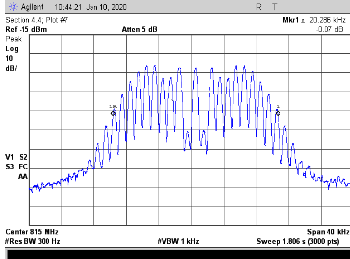
Input Signal to Amp; FM 16K
