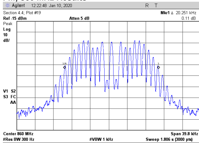
Input Signal to Amp; 300 Hz, FM 16K
