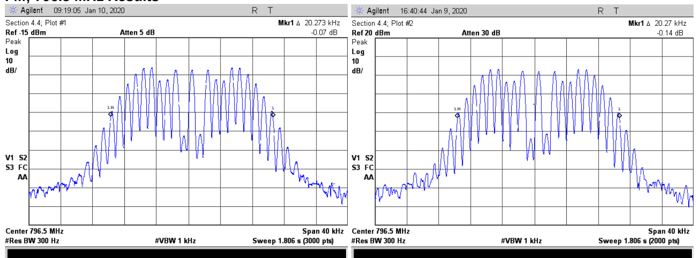
Input Signal to Amp; FM 16K
