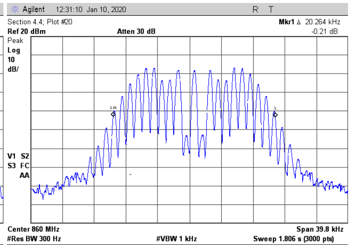
Amp output, Below AGC, FM 16K
