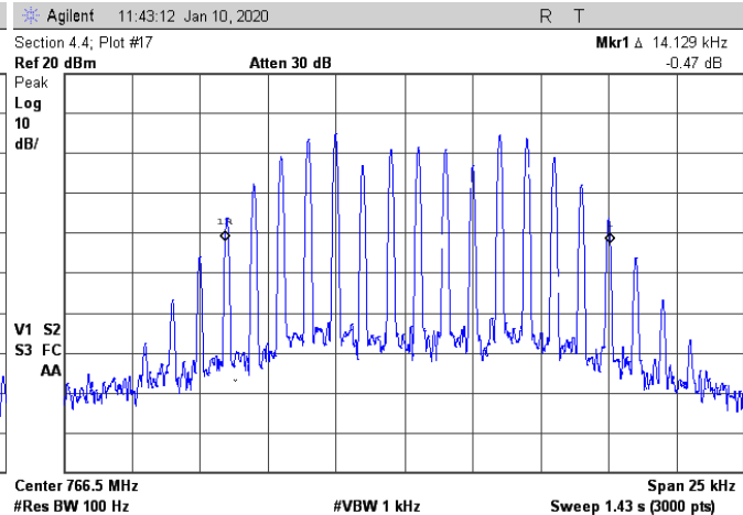
AMP Output: Below AGC, FM 11K
