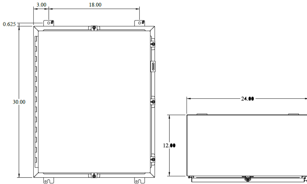
Figure: WST021 dimensions
