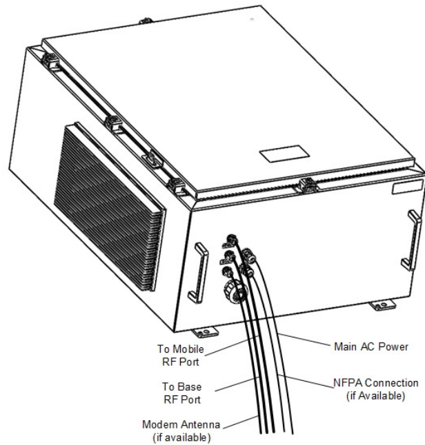
Figure: WST021 Configuration
