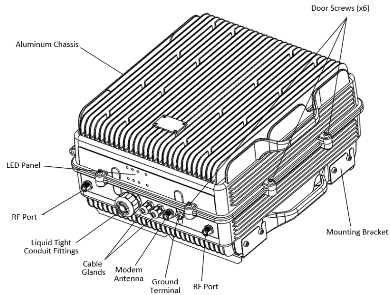
Figure: VHF "2 Port" Duplexed Configuration
