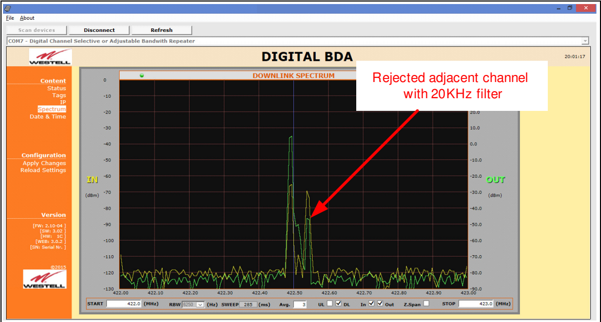
Adjacent channel rejection with 20KHz filter
