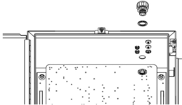
Figure: Remove the conduit connector
