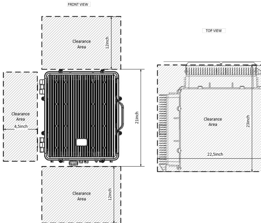
Figure: Mounting clearance WST012
