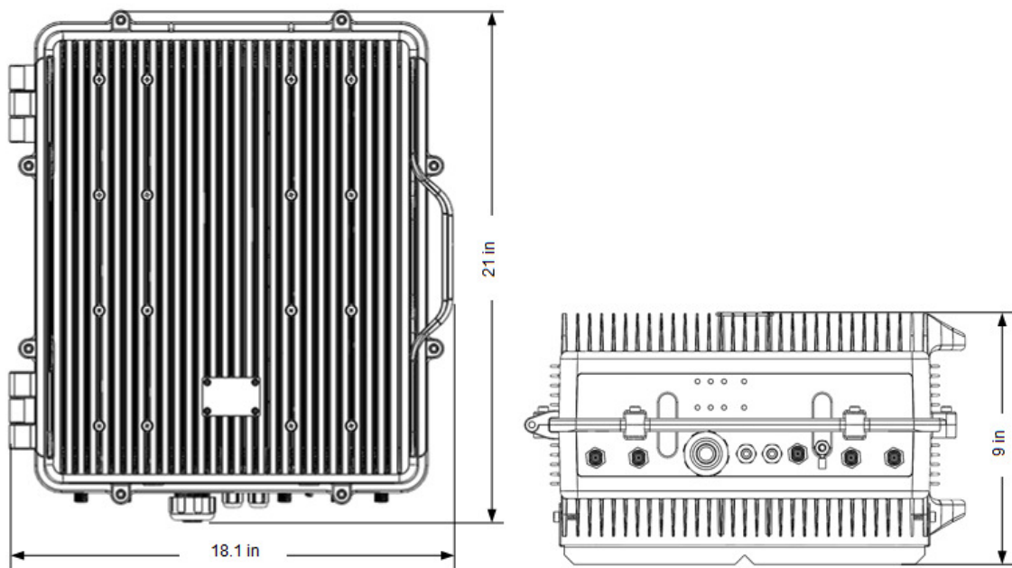
Figure: WST012 dimensions
