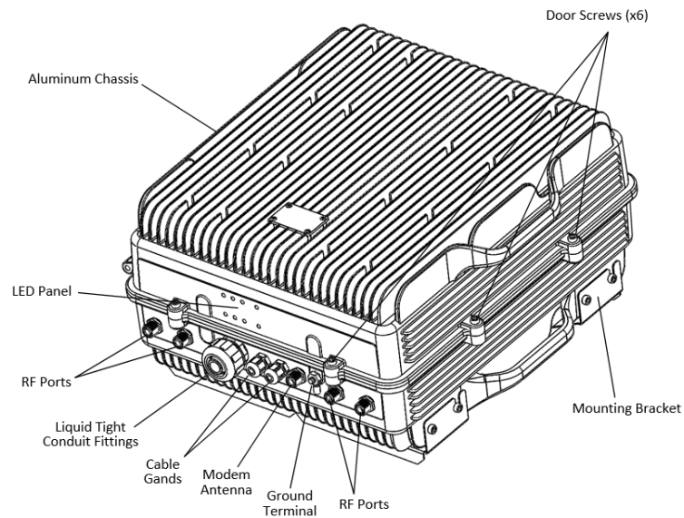
Figure: VHF "4 Port" Non-Duplexed Configuration
