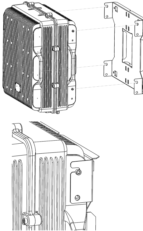
Figure: Hang the Signal Booster
