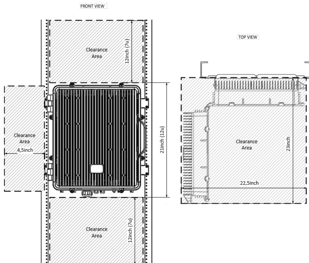
Figure: Mounting clearance for the rack mount option WST012
