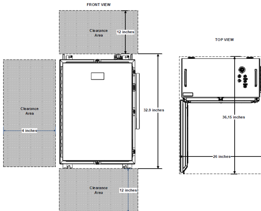
Figure: Mounting clearance WST021
