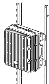
Mount and Fix the Signal Booster to the bracket.
