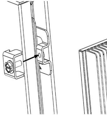
Figure: Secure Signal Booster cover
