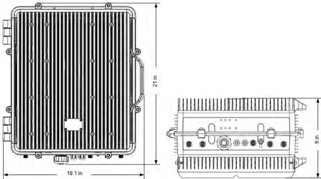
Figure: WST012 dimensions
