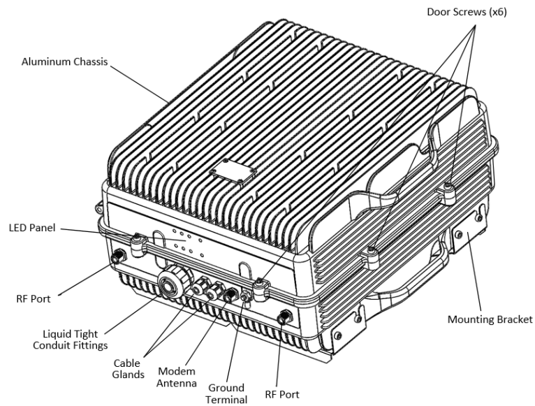
Figure: UHF "2 Port" Duplexed Configuration
