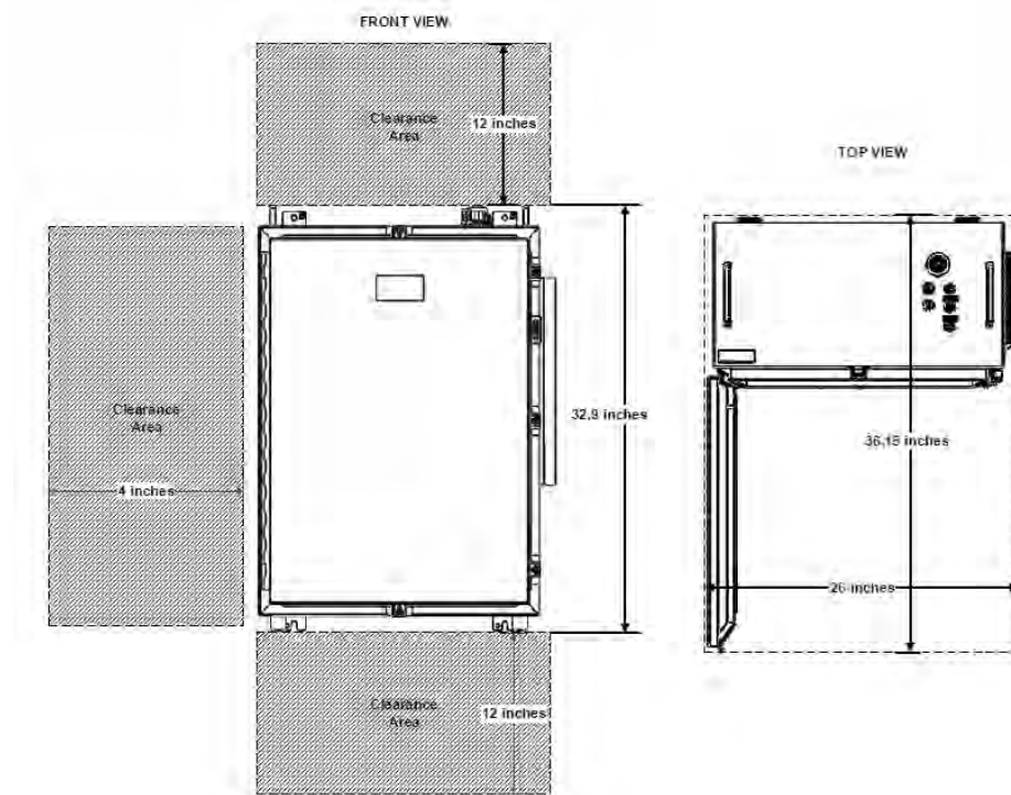
Figure: Mounting clearance WST021
