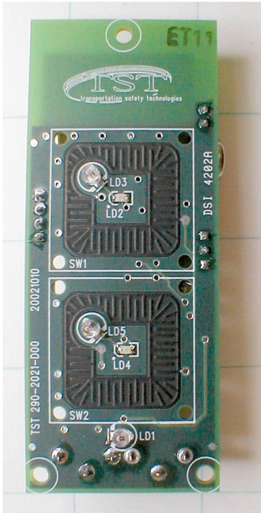
Bottom View of PCB
