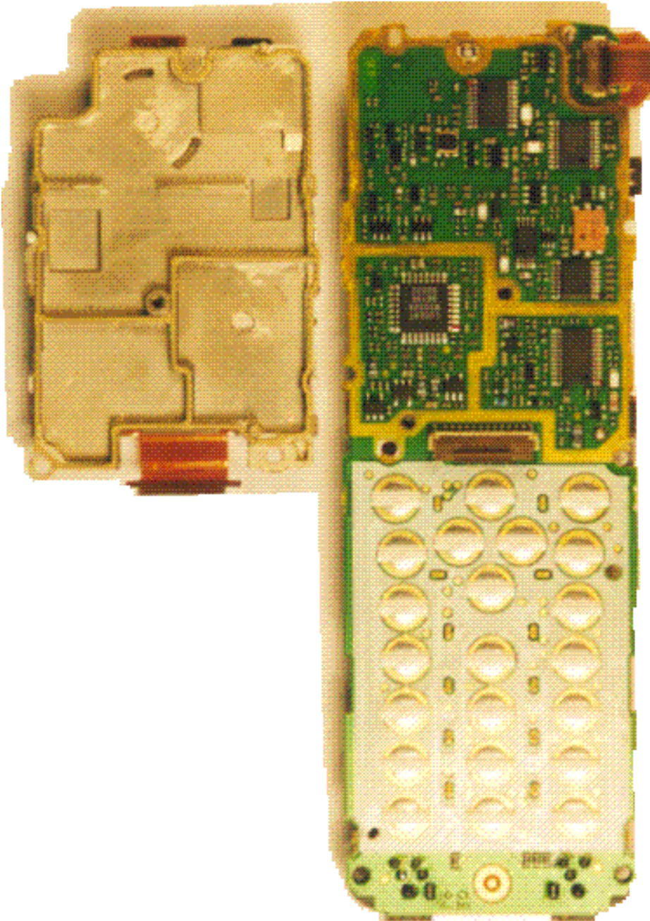
Front Side PCB with shield removed.
