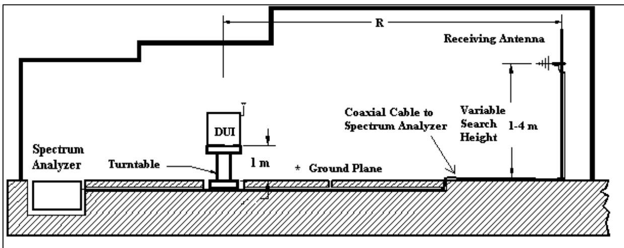
Set Up Figure 1 Effective Radiated Power (ERP)
