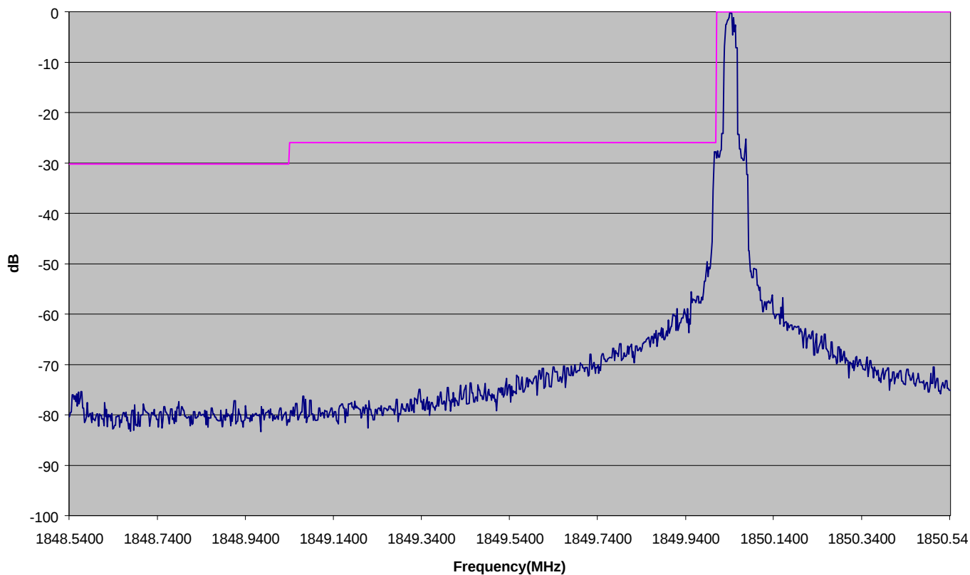
Out of Band Emissions - PCS Low Side < 1 MHz
