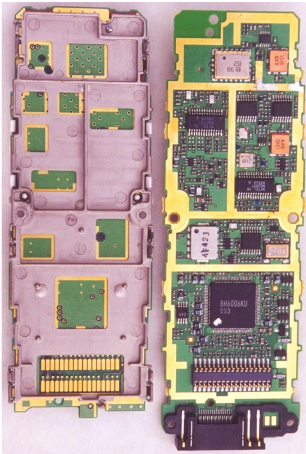
Front Side PCB with shield removed.
