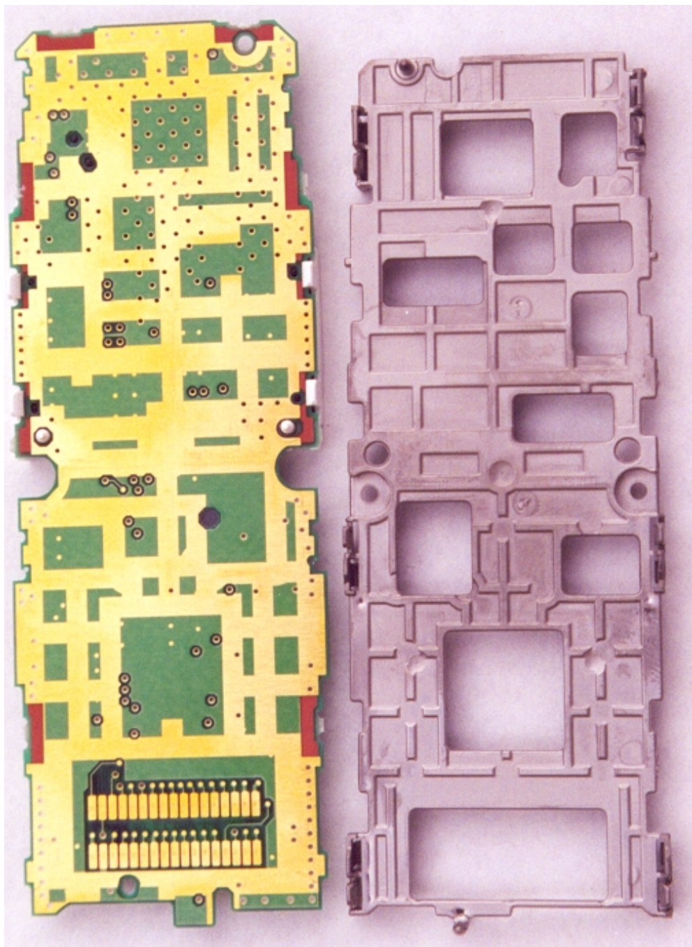
Front Side PCB with shield removed from Back
