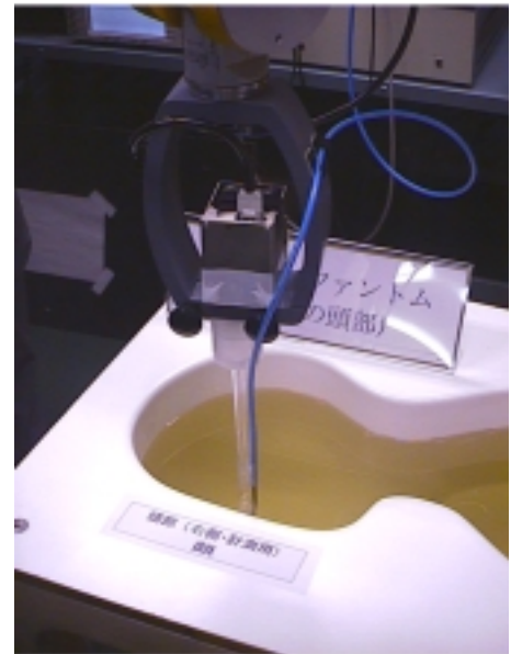
Fig2: The measurement set-up with a phantom containing tissue simulating liquid .
