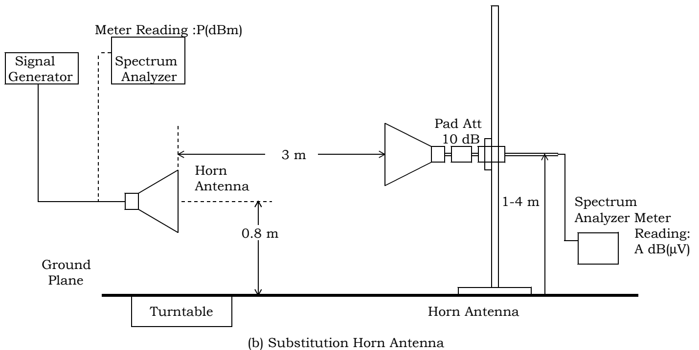
Fig.2 Maximum Transmitter Power (EIRP) Measurement(1900 MHz systems)
