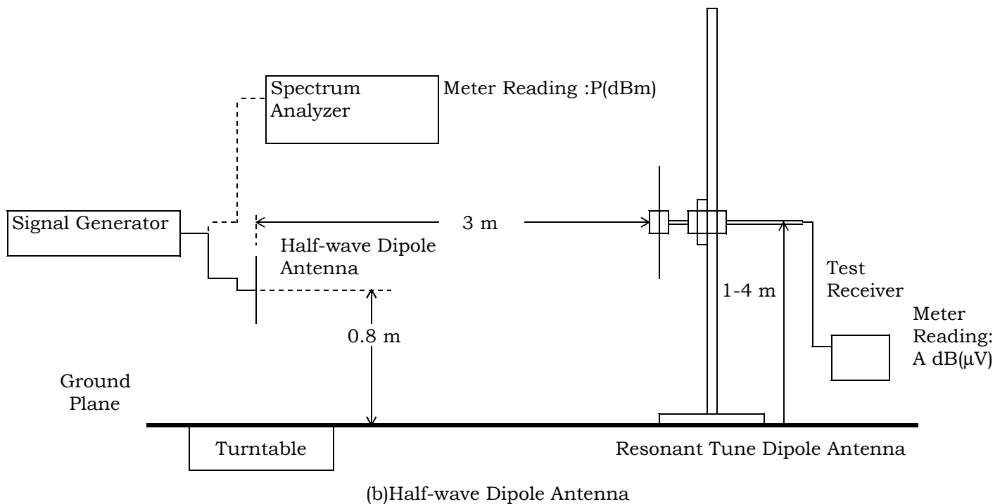
Fig.1 Maximum Transmitter Power(ERP) Measurement(800 MHz system)
