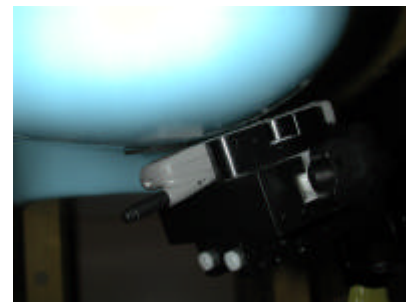
Figure 19. Head SAR Test Setup
