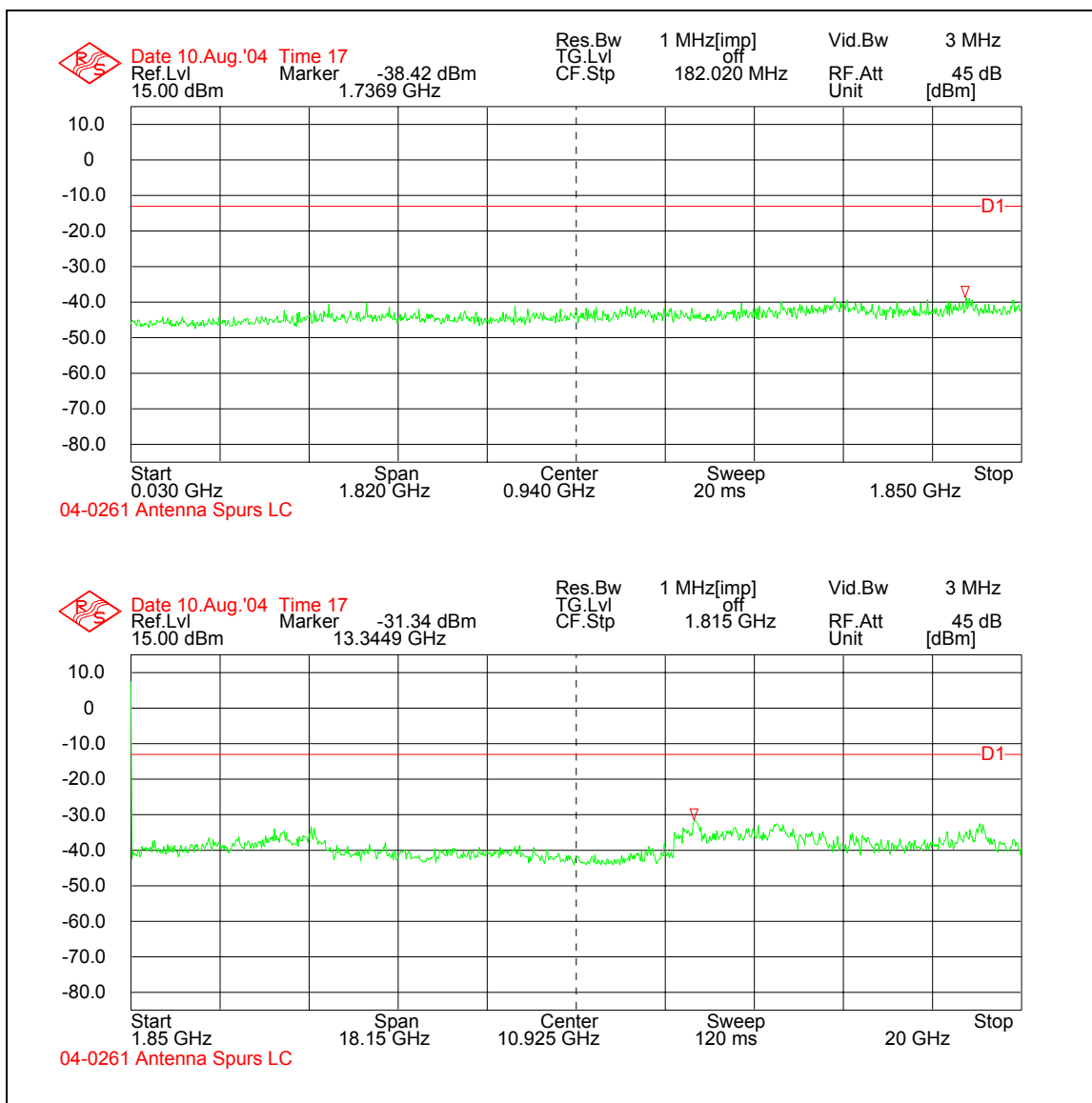
Figure 7.2.2-1: Low Channel
