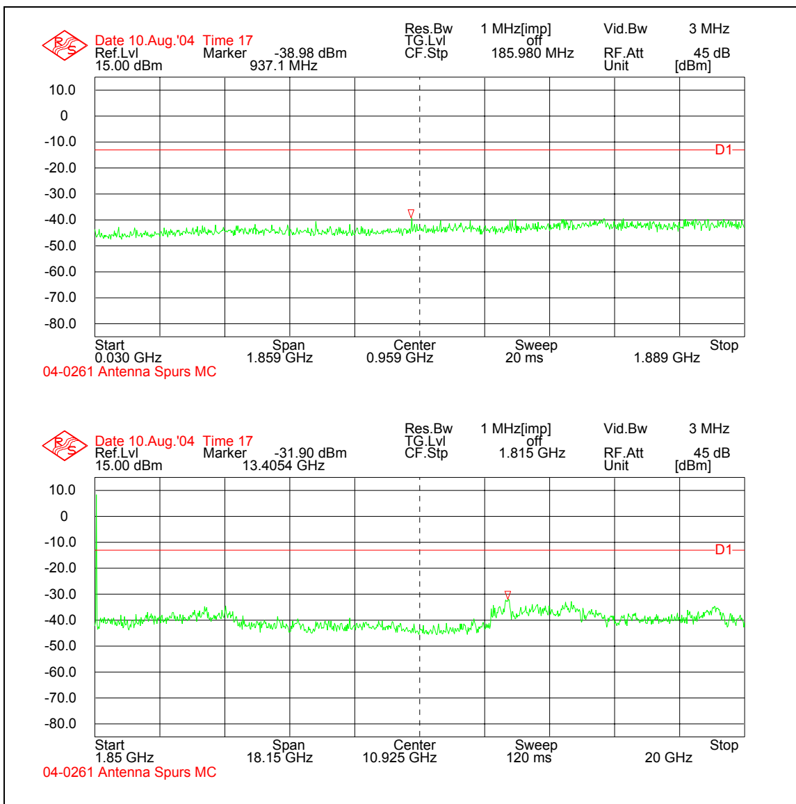
Figure 7.2.2-2: Middle Channel
