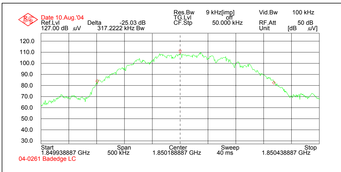
Figure 7.3.2-1: 26dB Bandwidth – Low Channel
