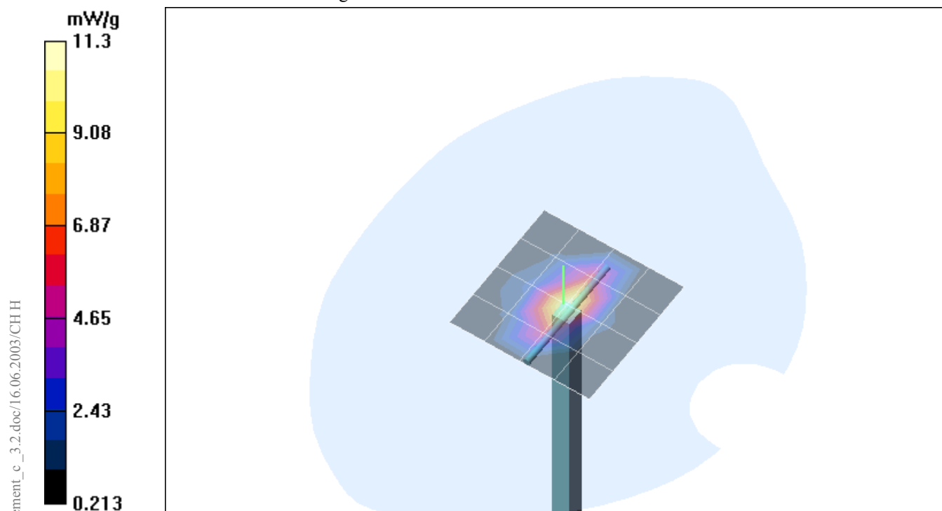
Fig. 11: Validation measurement 1900 MHz Head (September 01, 2003), coarse grid. Ambient Temperature: 20.9° C, Liquid Temperature: 20.1° C.
