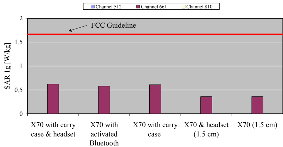
Fig. 10: The measured SAR values in body-worn configuration for the Panasonic X70 for PCS 1900 in comparison to the FCC exposure limit.
