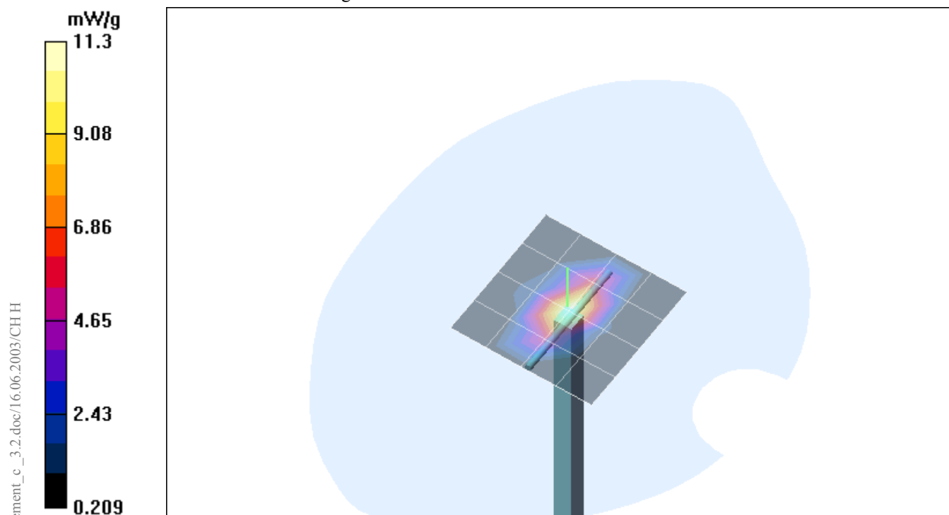
Fig. 12: Validation measurement 1900 MHz body (September 02, 2003), coarse grid. Ambient Temperature: 20.9° C, Liquid Temperature: 19.8° C.
