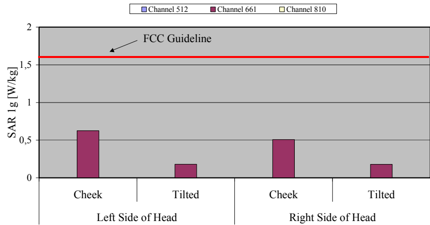
Fig. 9: The measured head phantom SAR values for the Panasonic X70 for PCS 1900 in comparison to the FCC exposure limit.
