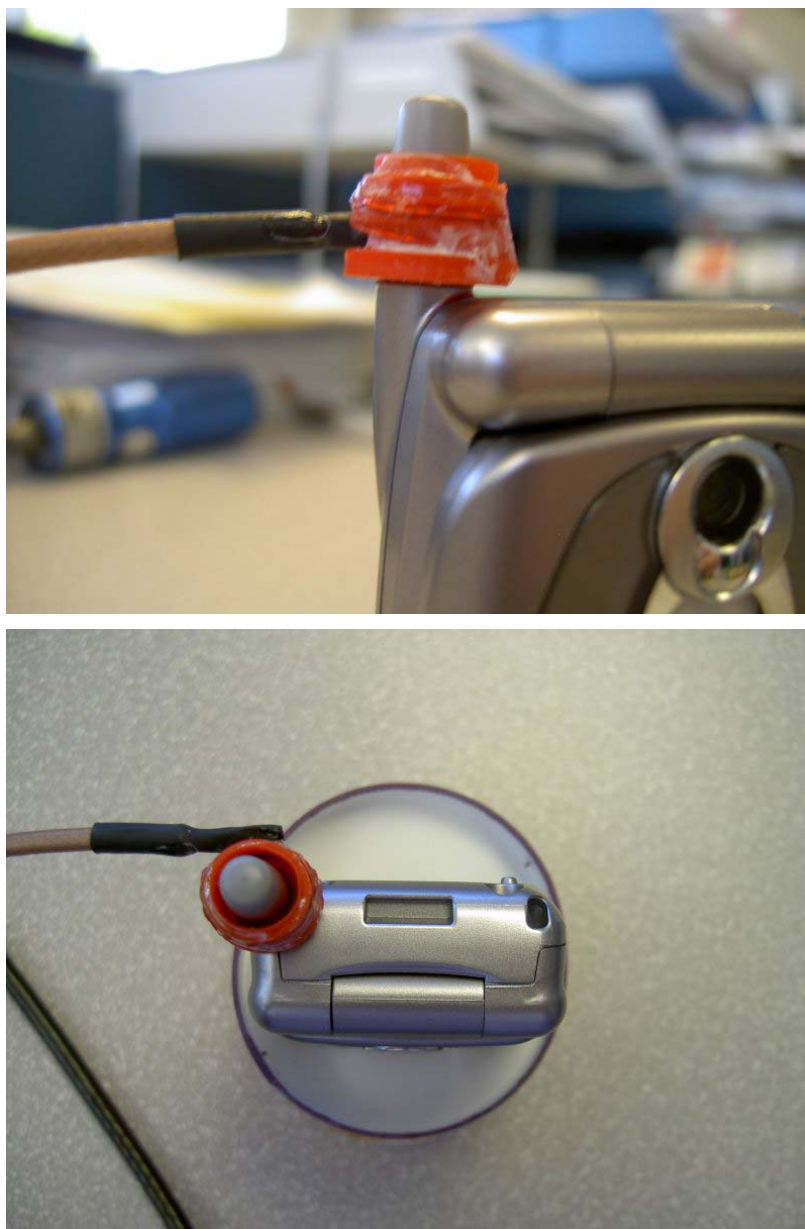
Fig. 8: Provided coupler to control the output power.
