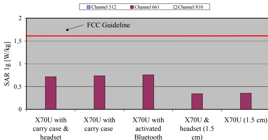
Fig. 13: The measured SAR values in body-worn configuration for the Panasonic X70U for PCS 1900 in comparison to the FCC exposure limit.
