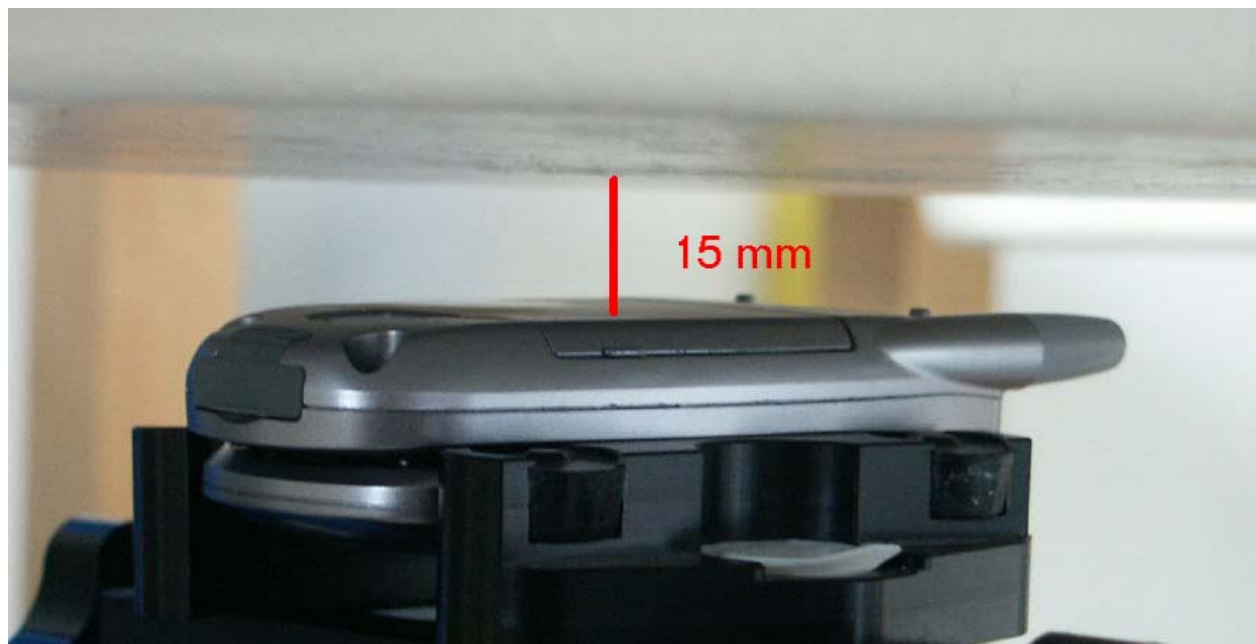
Fig. 31: Body worn configuration without headset and 1.5 cm distance (1 TX slot).
