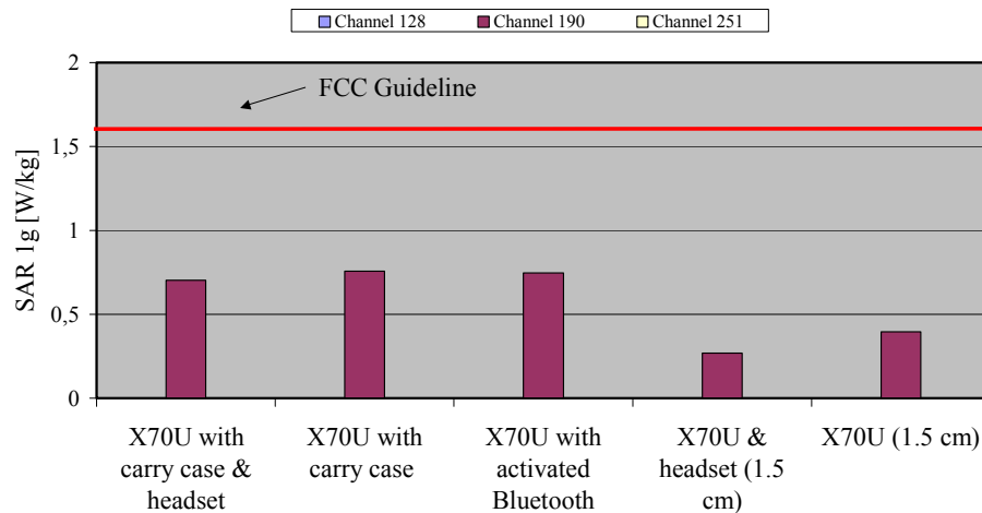
Fig. 12: The measured SAR values in body-worn configuration for the Panasonic X70U for GSM 850 in comparison to the FCC exposure limit.
