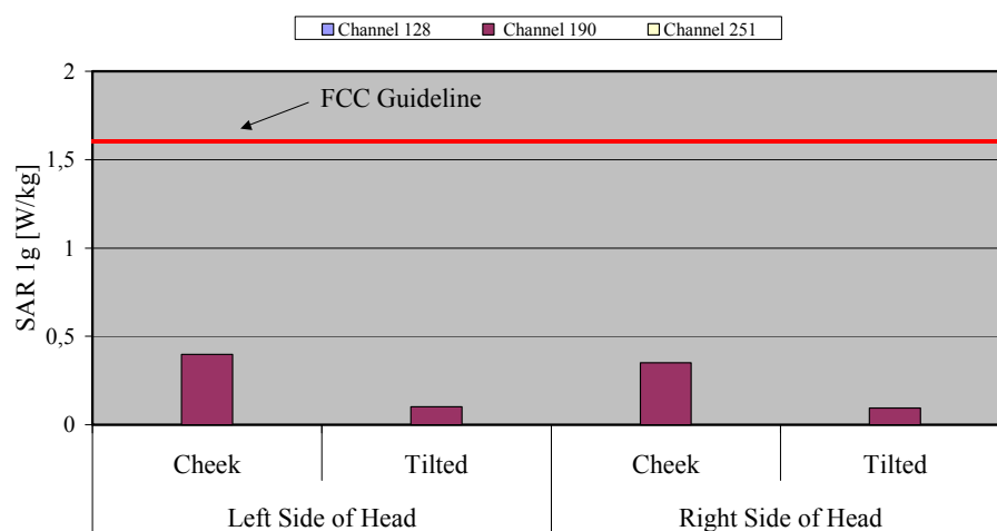
Fig. 10: The measured head phantom SAR values for the Panasonic X70U for GSM 850 in comparison to the FCC exposure limit.
