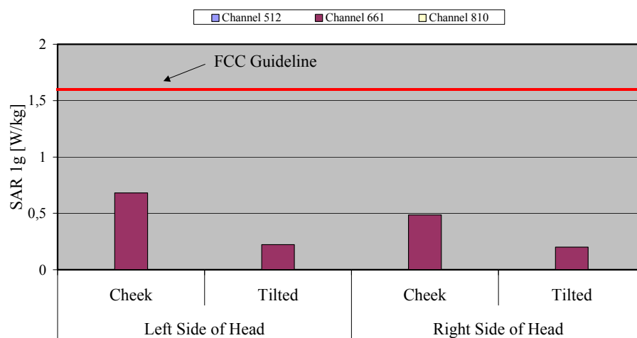
Fig. 11: The measured head phantom SAR values for the Panasonic X70U for PCS 1900 in comparison to the FCC exposure limit.
