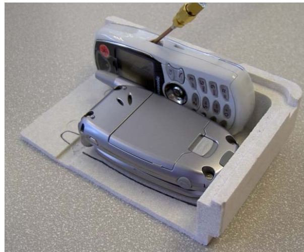
Fig. 9: Provided coupler to control the output power, position for PCS 1900.
