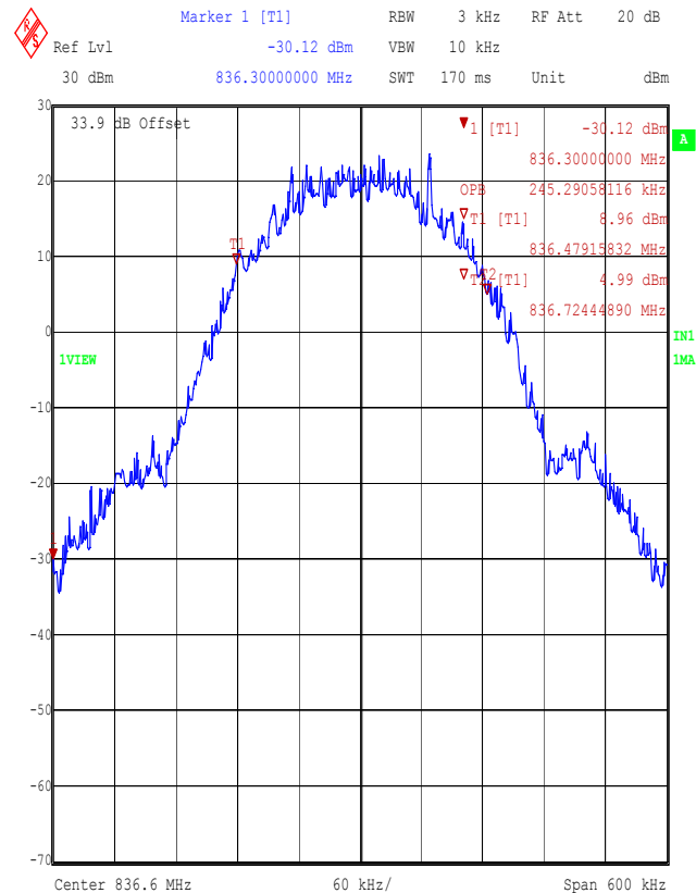
Middle Channel
