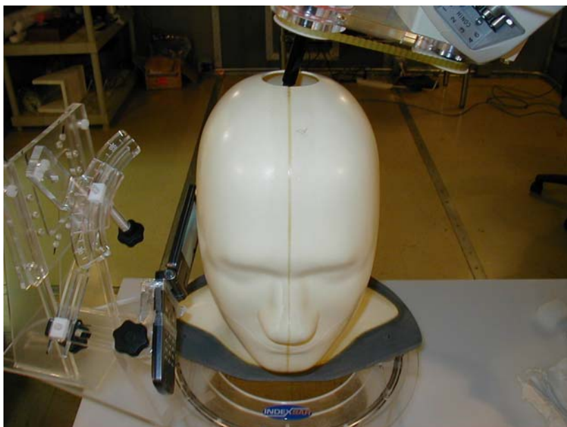
Figure S2. Setup Configuration of Right Ear Cheek and Tilt ( 1900 Head SAR)
