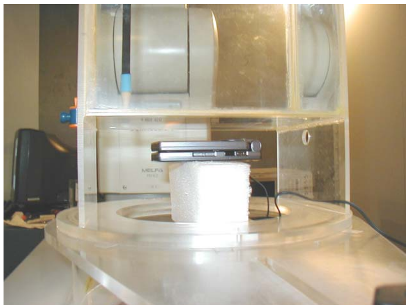
Figure S3. Setup Configuration of Body SAR
