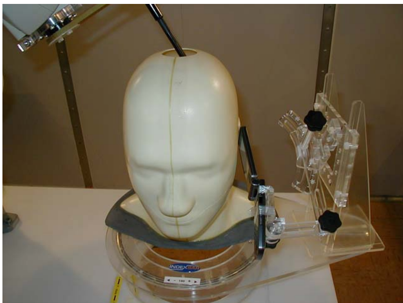
Figure S1. Setup Configuration of Left Ear Cheek and Tilt ( 1900 Head SAR)
