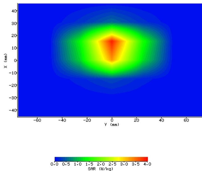
Validation Measurement – 1800 MHz in Head tissue
