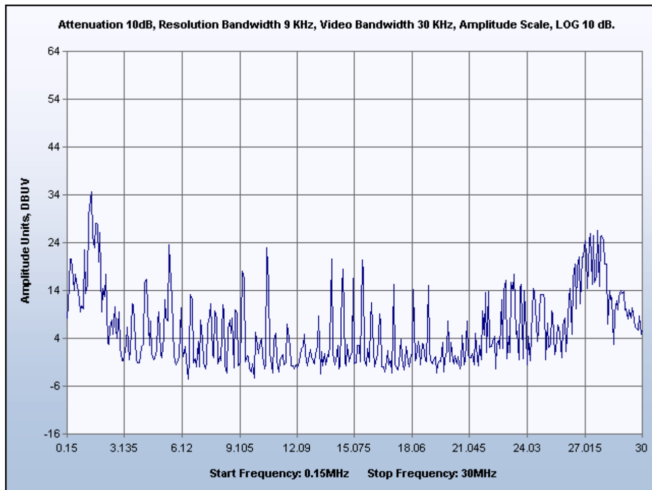
Graph 1. Conducted Emissions, Phase Plot
