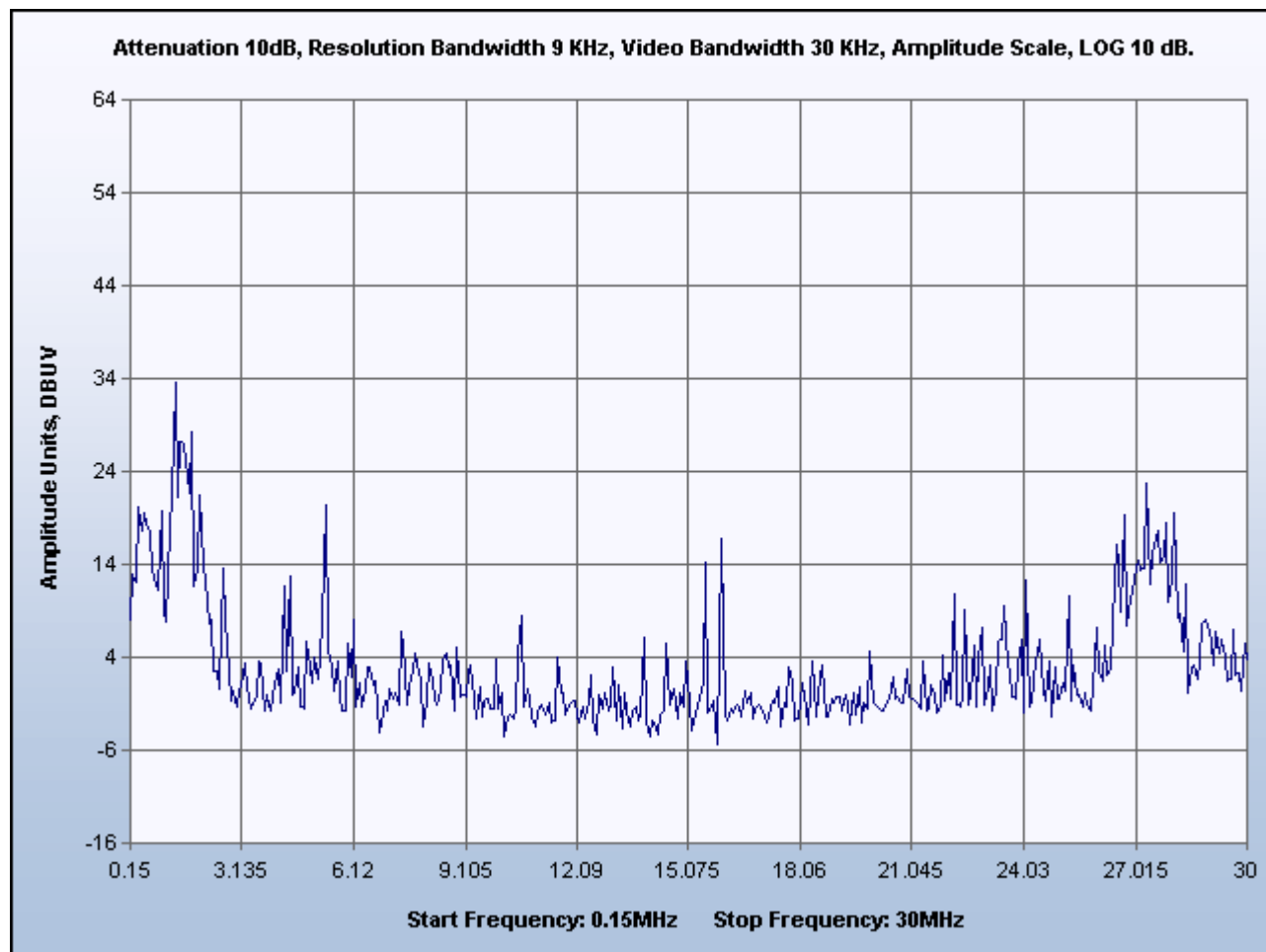
Graph 2. Conducted Emissions, Neutral Plot
