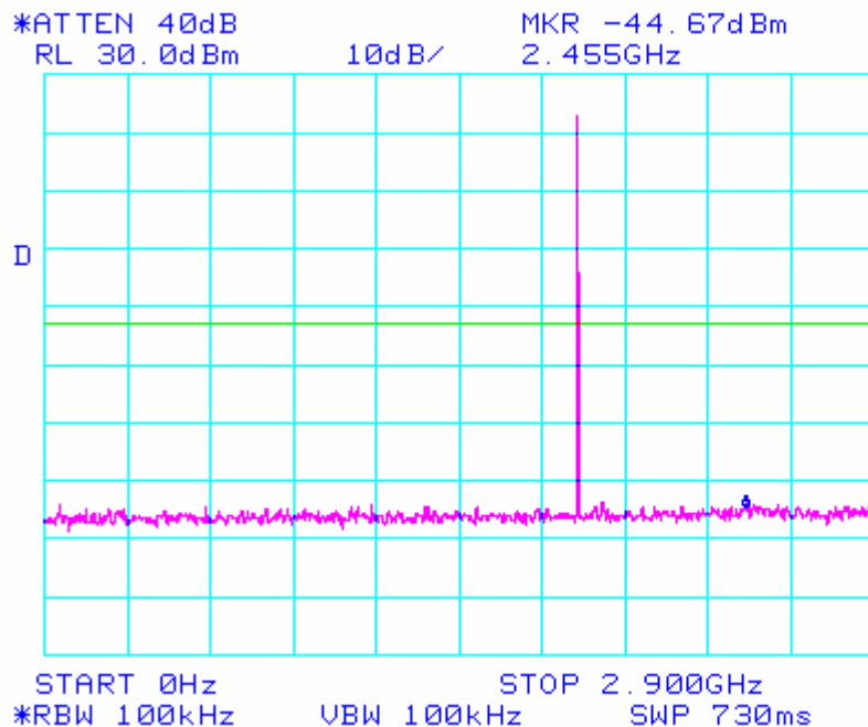
Plot 4 Conducted Spurious Emissions Measurements at Antenna Terminals Test Results
