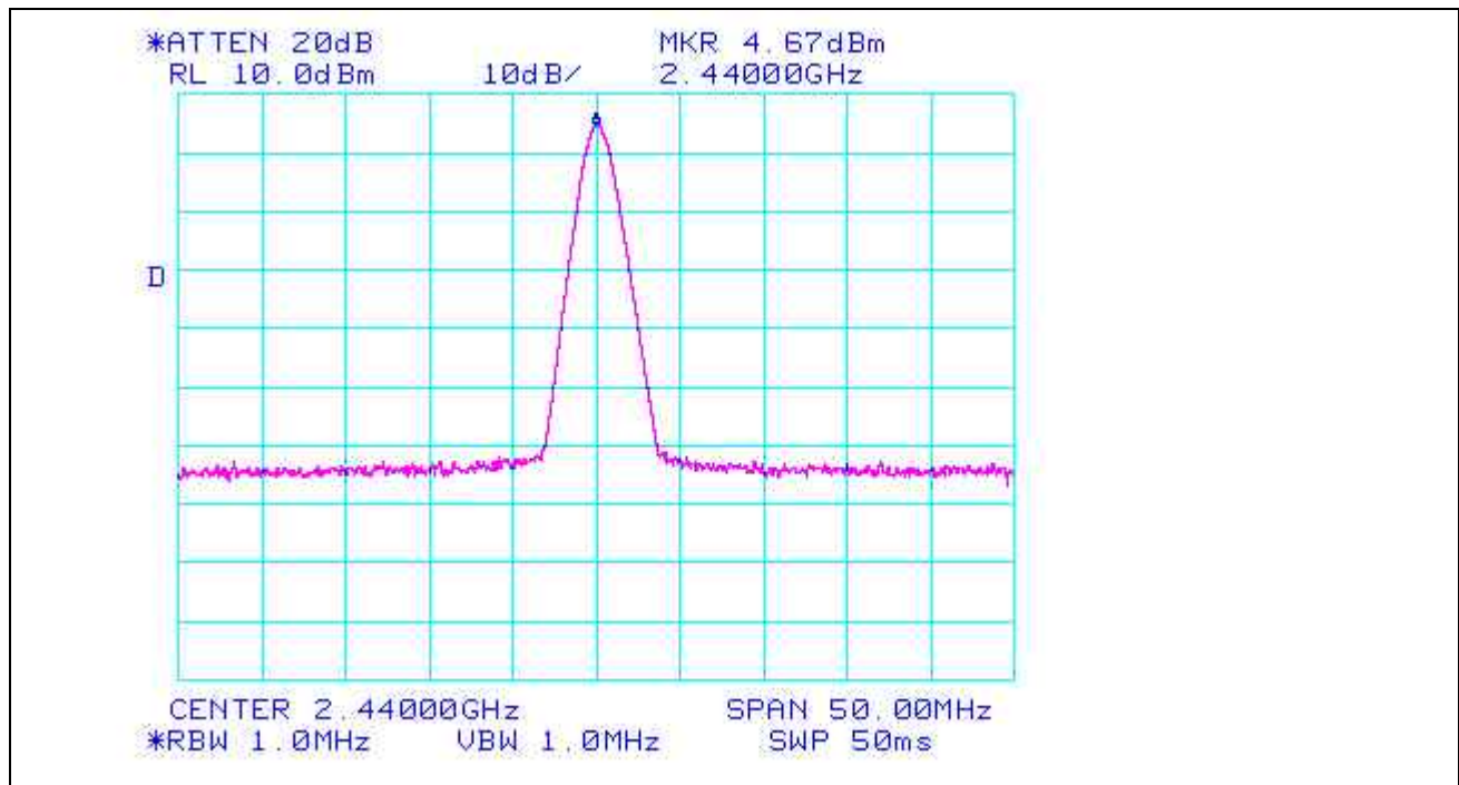
Graph 5. Peak Power Output, Test Results, Medium
