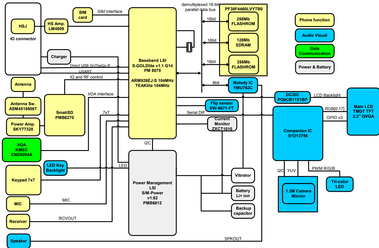
EB-VS3 System Block Diagram
