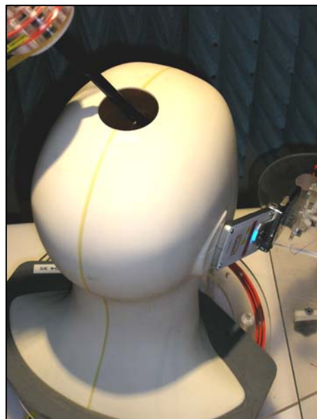
Figure 20: Positional photograph of the Panasonic EB-VS3 Handset in the Right-hand 15° Position
