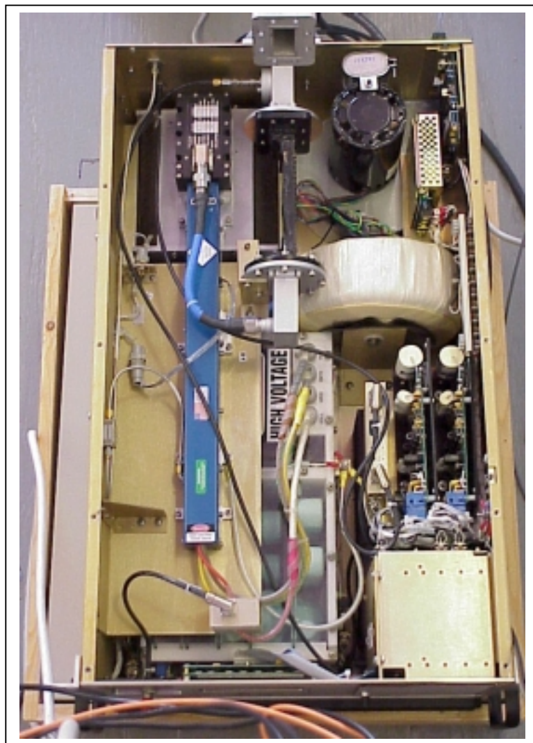
Figure 3 TWT Amplifier - Top Cover Removed
