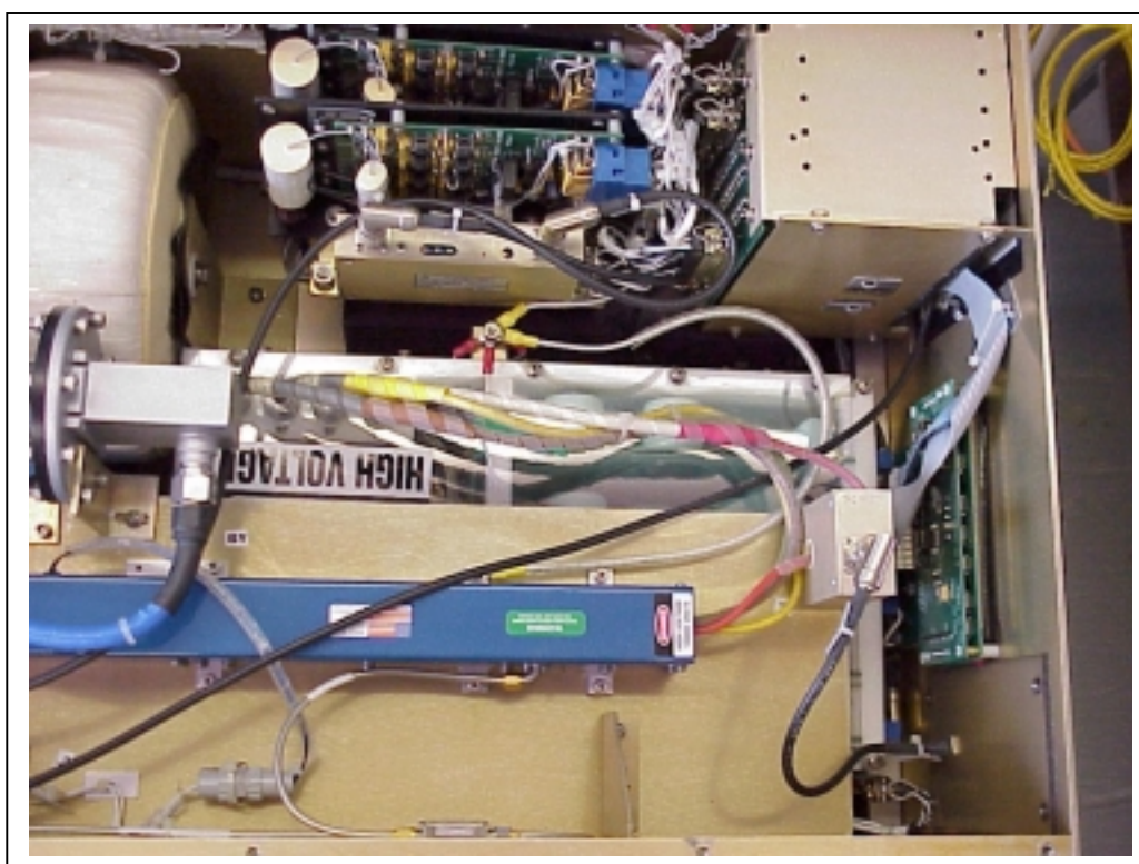
Figure 2 Traveling Wave Tube - High Voltage Supply
