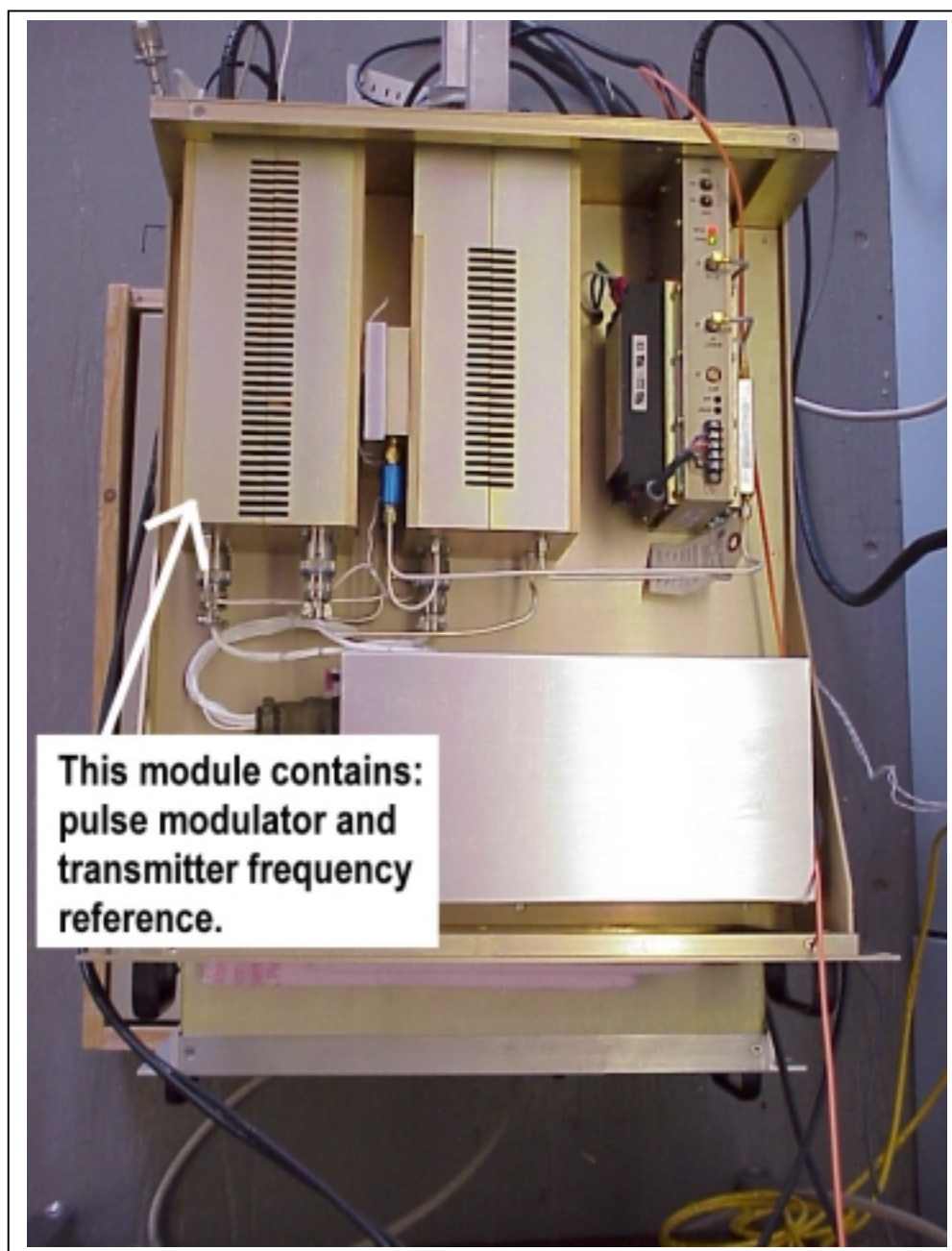
Figure 6 Receiver - Top Cover Removed
