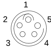
Figure iii : 5 Pin LEMO pin out orientation viewed from solder spill side
