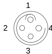
Figure ii : 4 Pin LEMO pin out orientation viewed from solder spill side
