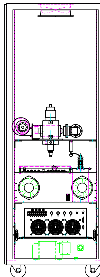
REAR ELEVATION [PANELS REMOVED]
