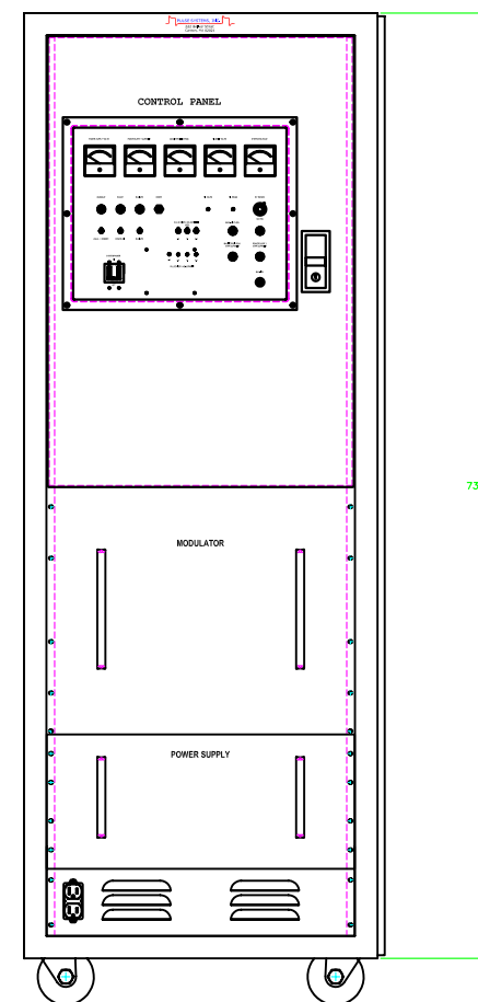
FRONT ELEVATION (DOOR & PANELS ON)
