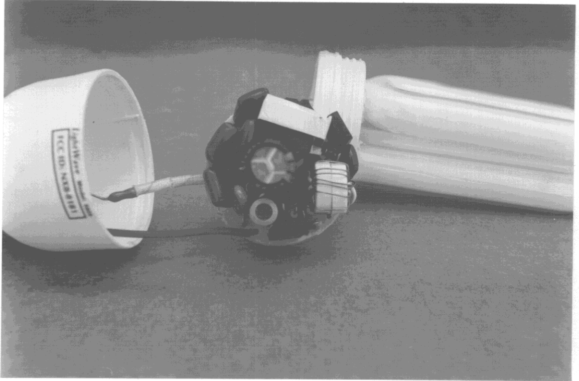
4.12 Photo: 9809 Printed Circuit Board - Top View
