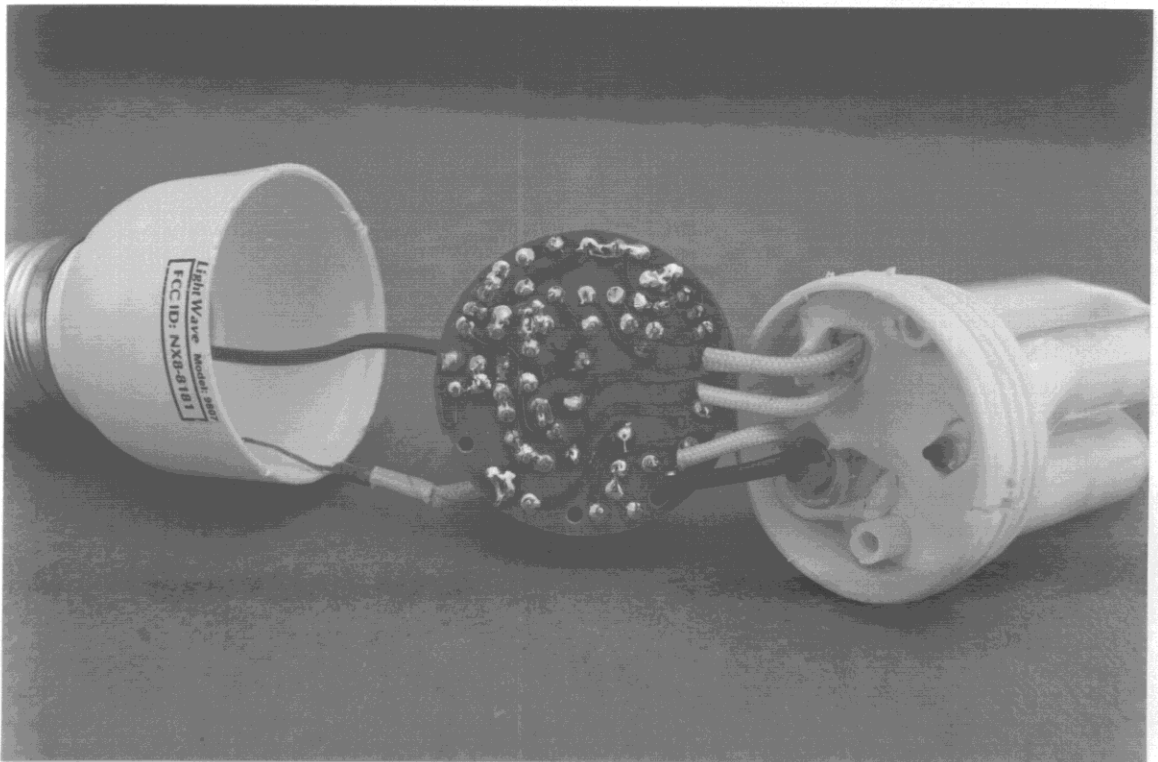
4.16 Photo: 9807 Printed Circuit Board - Bottom View
