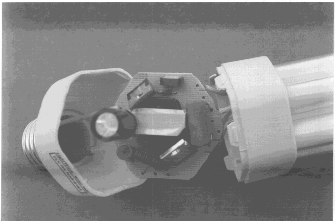
4.6 Photo: 9832 (9826) Printed Circuit Board - Top View
