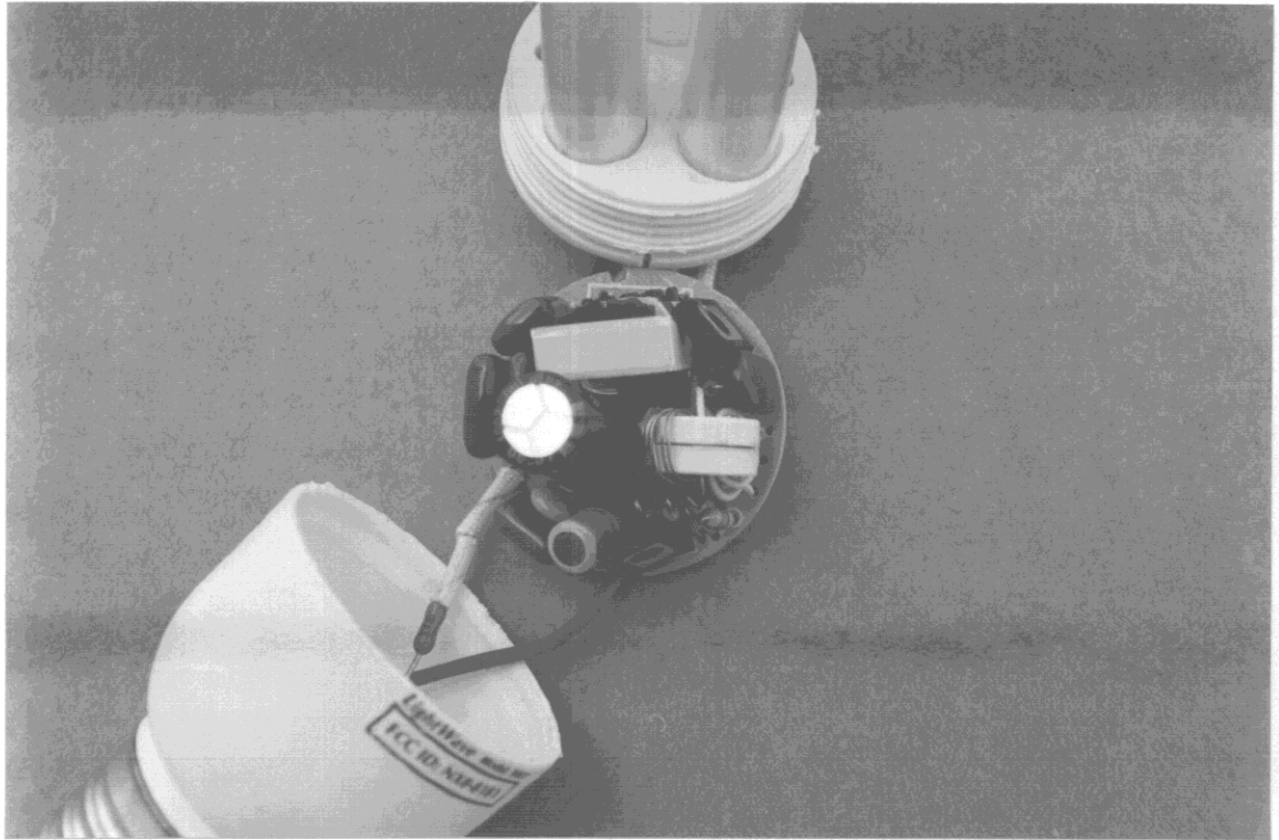
4.15 Photo: 9807 Printed Circuit Board - Top View
