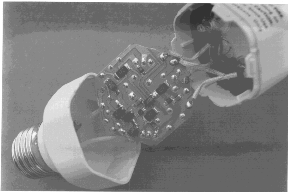
4.7 Photo: 9832 (9826) Printed Circuit Board - Bottom View
