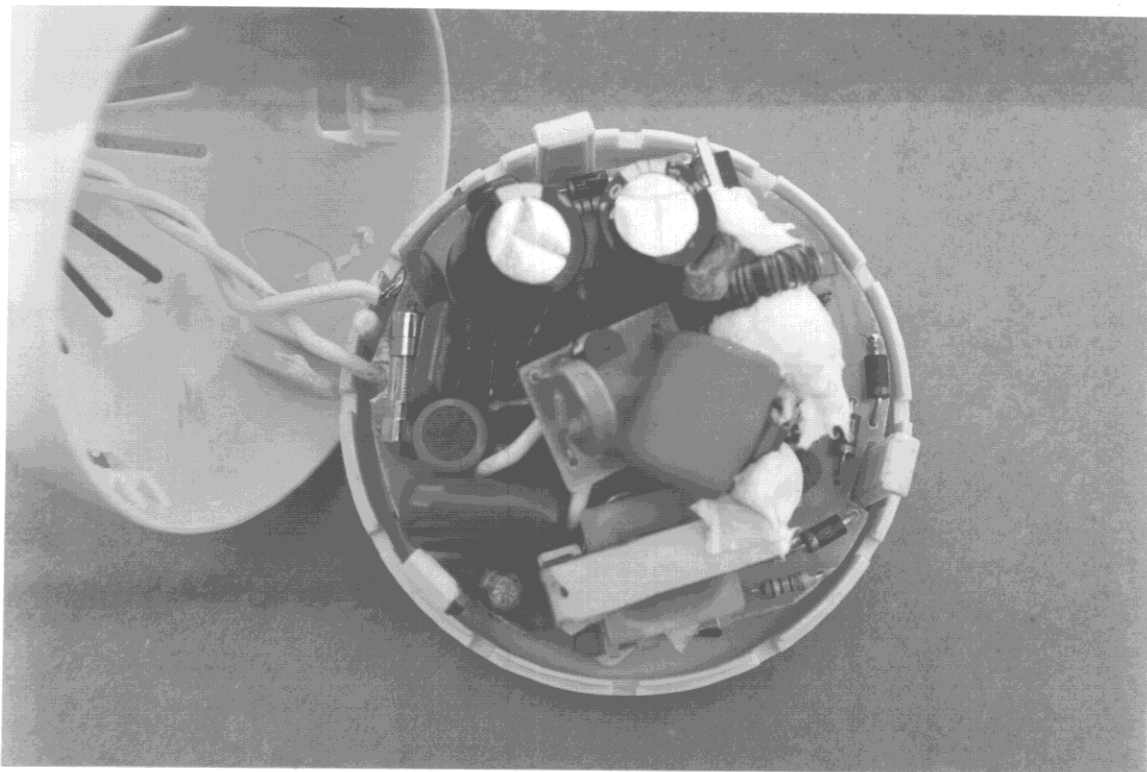
4.3 Photo: 9855 (9838) Printed Circuit Board - Top View
