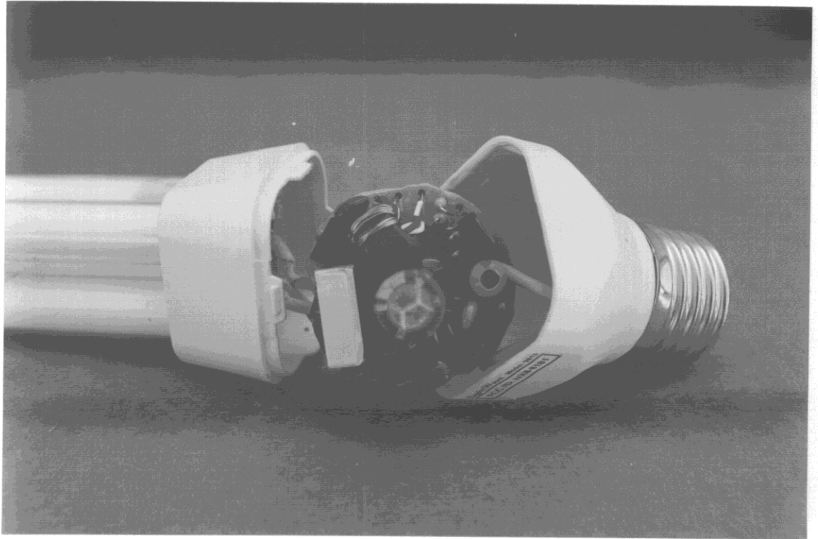
4.9 Photo: 9813 Printed Circuit Board - Top View
