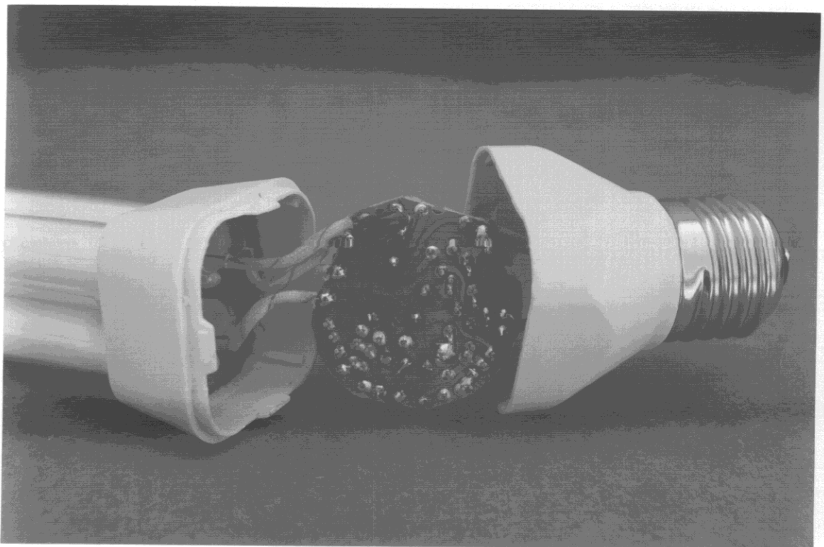
4.10 Photo: 9813 Printed Circuit Board - Bottom View
