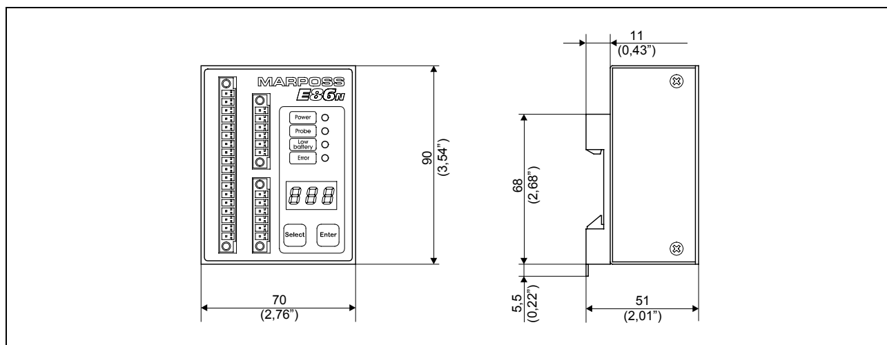
Figure 9-2. Overall dimensions.
