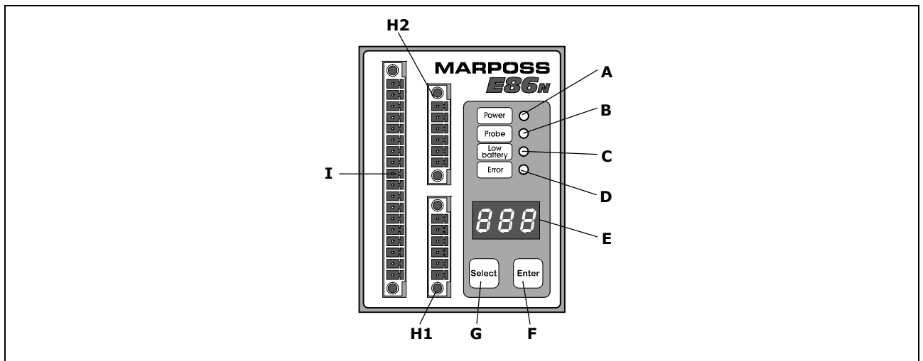
Figure 9-1: Front panel.
