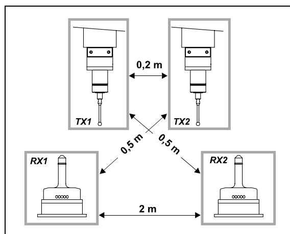
Figure 6-2. Distances when using more than one system.
