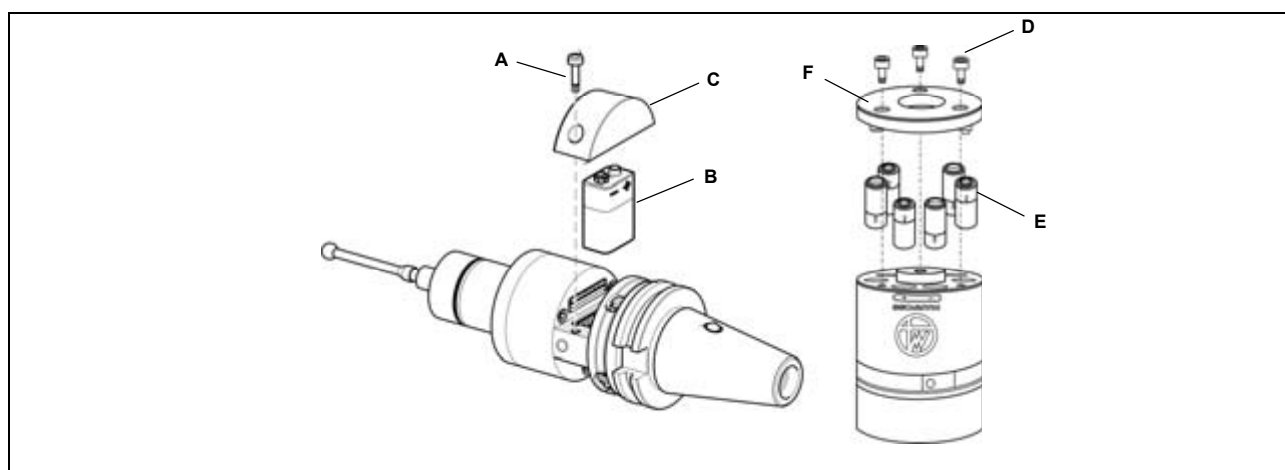
Figure 15-1. Inserting/changing the batteries
