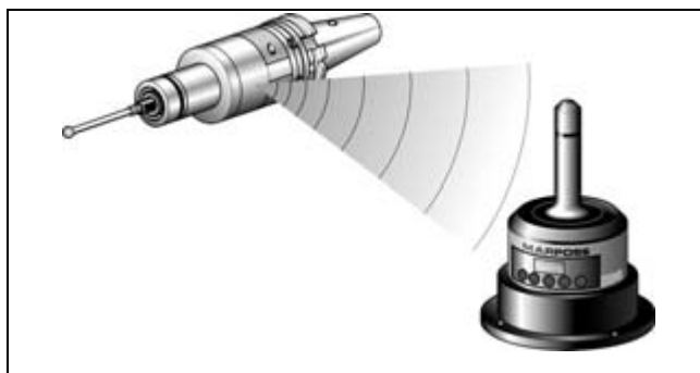
Figure 6-3. Radio activation.
