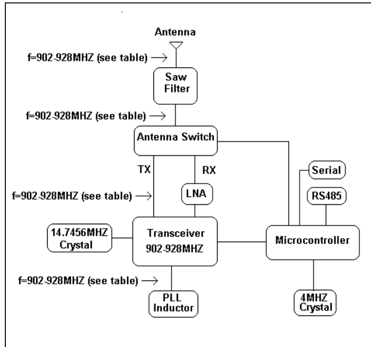
900MHz Transceiver Block Diagram
