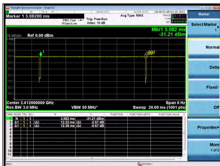
Fig-4.1 WLAN2.4G_802.11b Duty cycle
