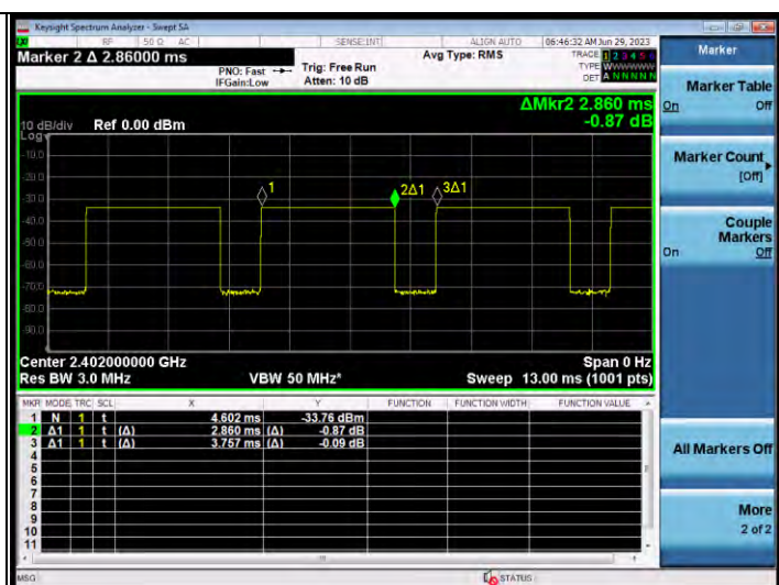
Fig-4.2 BT_GFSK Duty cycle
