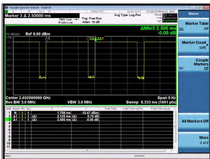
Fig-4.3 BLE_1Mbps Duty cycle
