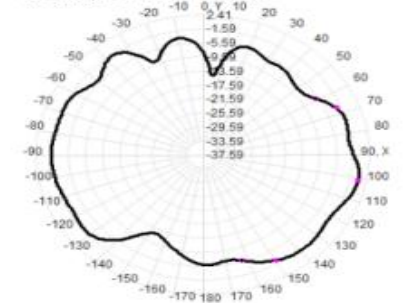
Total(H+XY), Max= 0.11dBi, CrD=14.97
