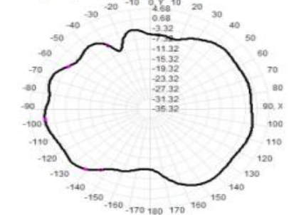
Total(H+XY), Max=-0.12dBi, CrD=11.15
