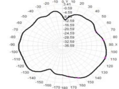
Total(H+XY), Max=-0.11dBi, CrD=11.77
