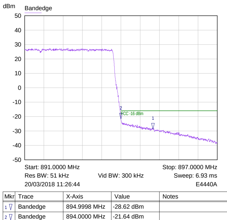
51kHz RBW plot
