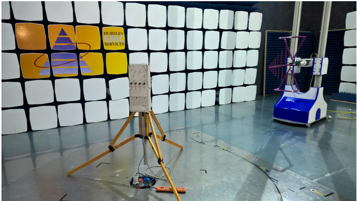
Radiated Spurious Emissions: 30-1000 MHz
