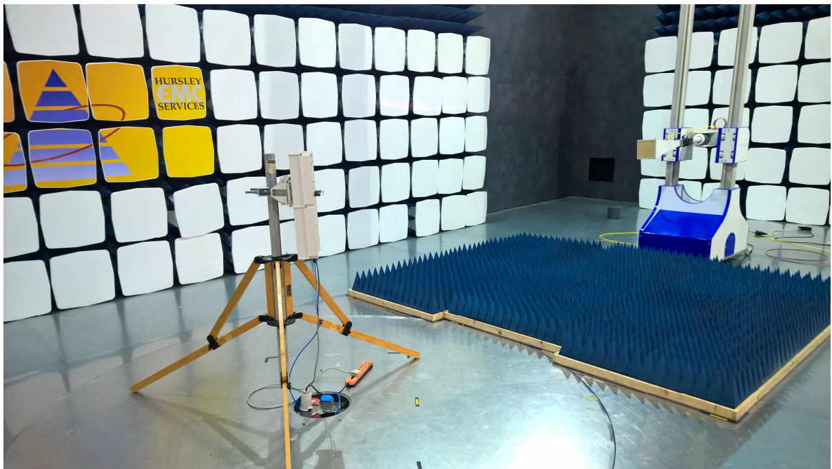
Radiated Spurious Emissions: 1-18 GHz
