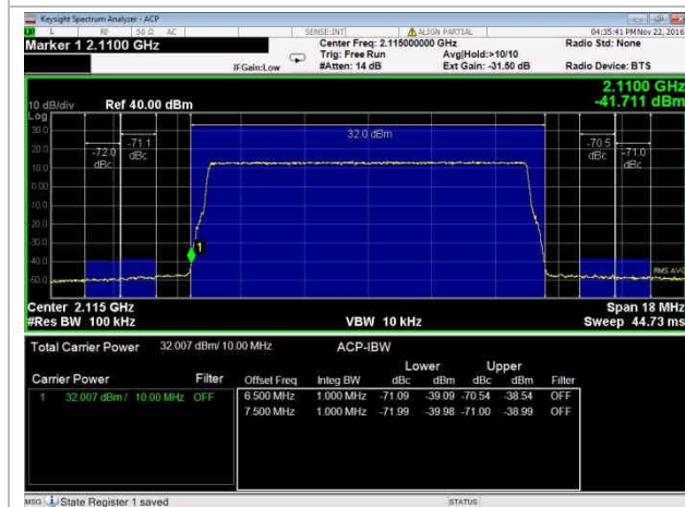
10 MHz Channel, 64 QAM, low
