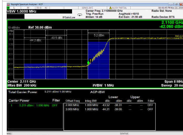
20 MHz Channel, 64 QAM, low
