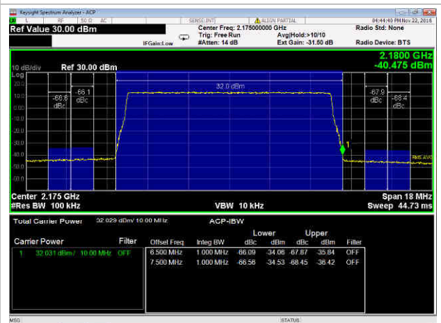
10 MHz Channel, 64 QAM, high
