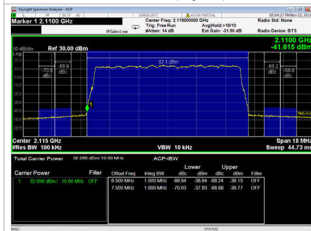
10 MHz Channel, 16 QAM, low
