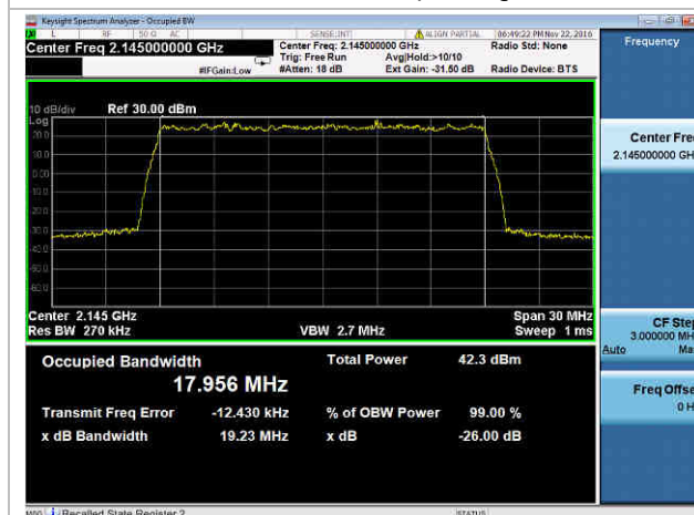
20 MHz Channel, 16 QAM
