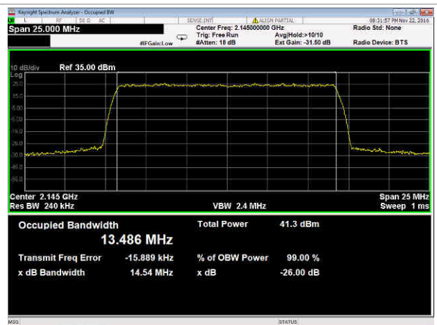
15 MHz Channel, 64 QAM
