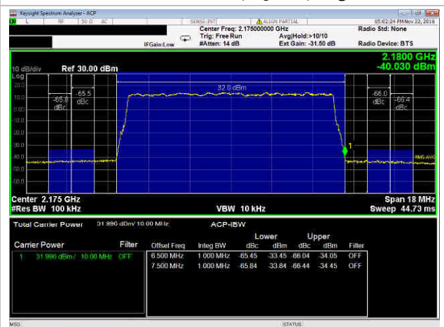
10 MHz Channel, 16 QAM, high
