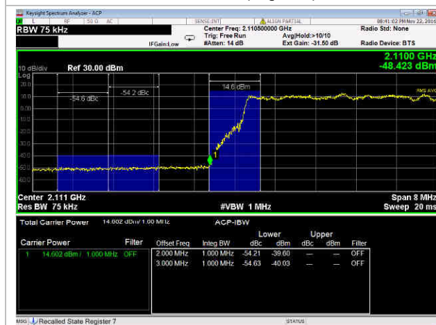
15 MHz Channel, 16 QAM, low
