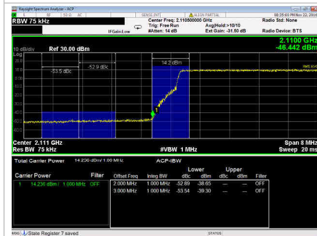
15 MHz Channel, 64 QAM, low
