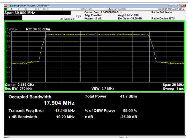
20 MHz Channel, 64 QAM
