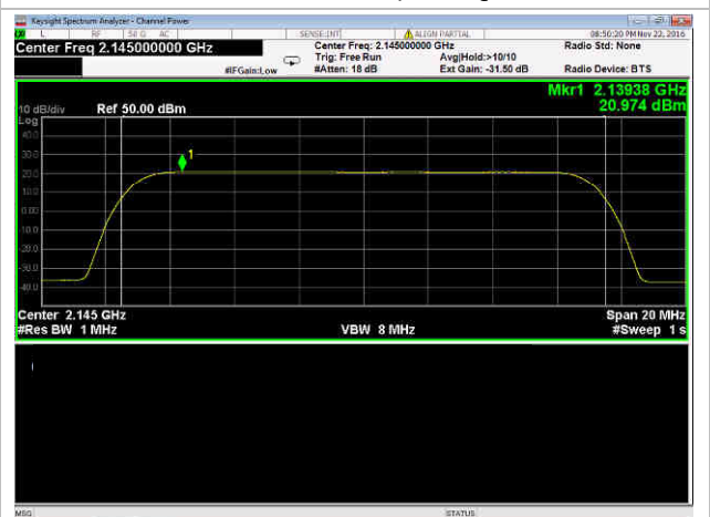
15 MHz Channel, QPSK
