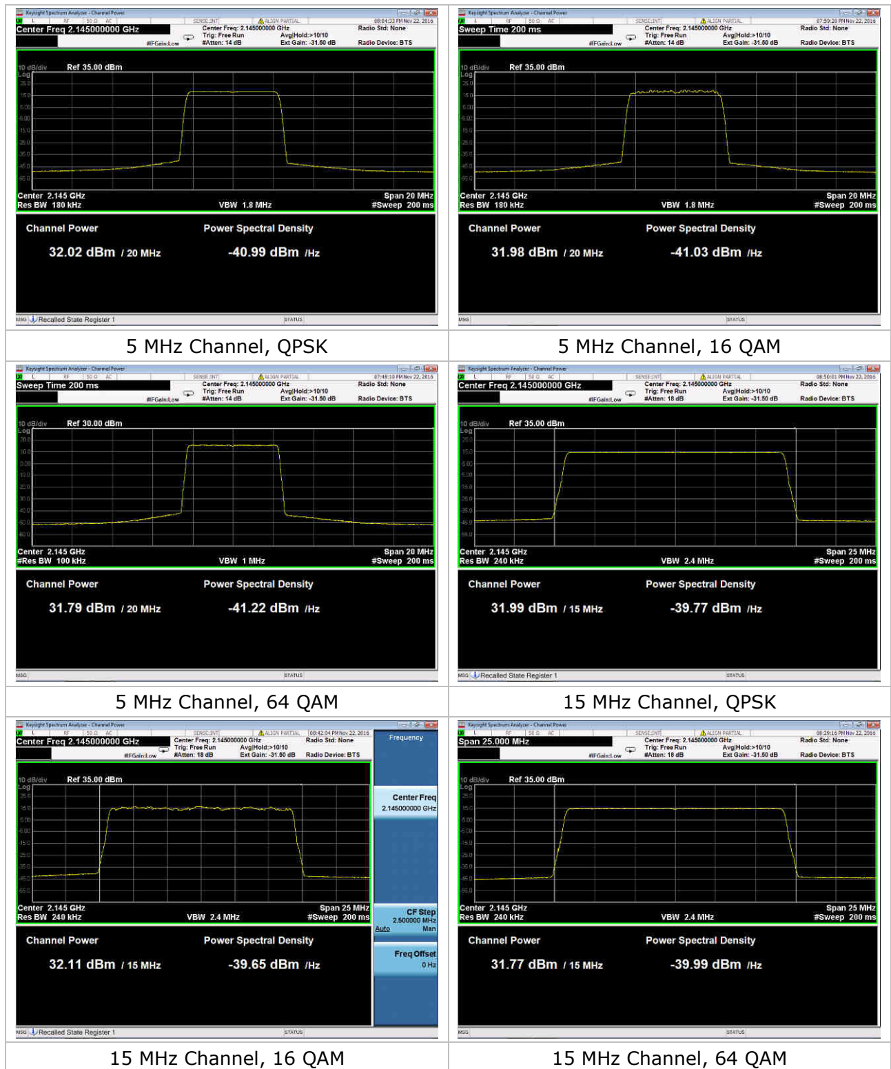
Figure 3: Transmit Power plots for centre channel
