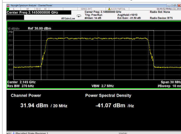
20 MHz Channel, 16 QAM
