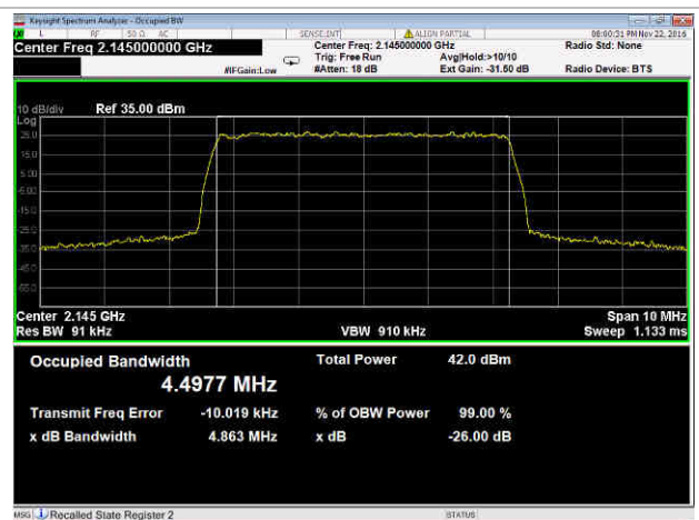
5 MHz Channel, 16 QAM
