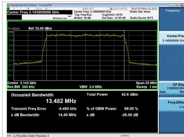
15 MHz Channel, 16 QAM
