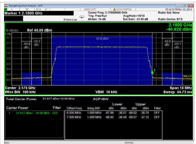
10 MHz Channel, QPSK, high
