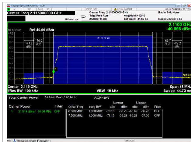
10 MHz Channel, QPSK, Low
