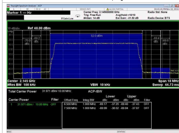
10 MHz Channel, 64 QAM
