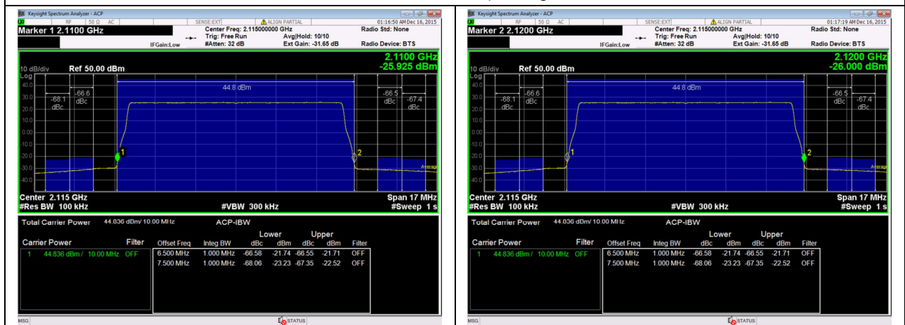
10 MHz Channel, 64 QAM
