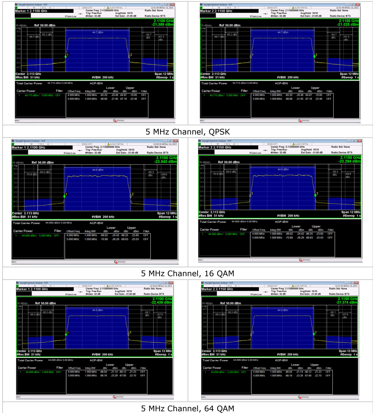
Figure 1: Transmit Power and band edge plots; 5 MHz channel
