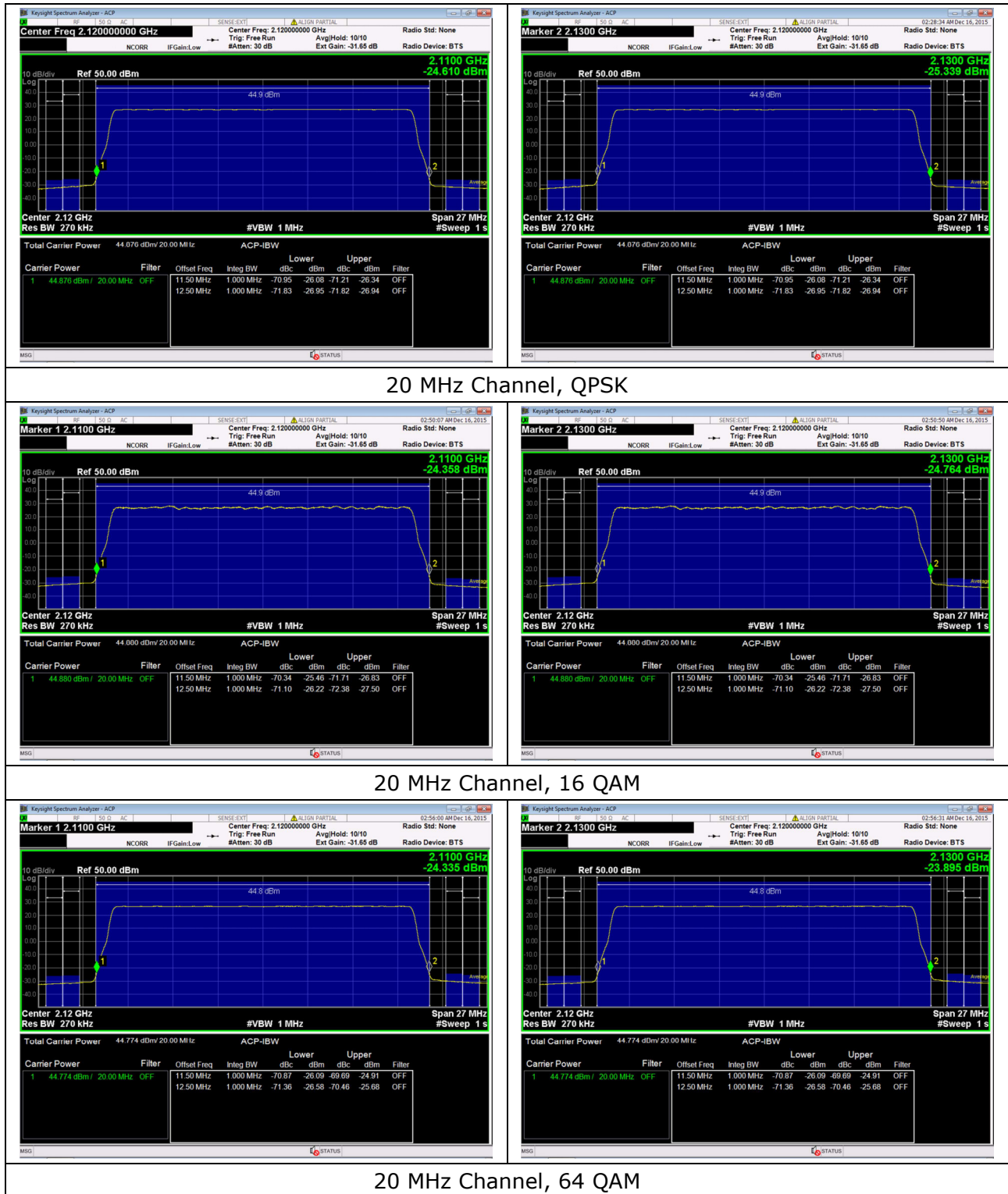
Figure 4: Transmit Power and band edge plots; 20 MHz channel
