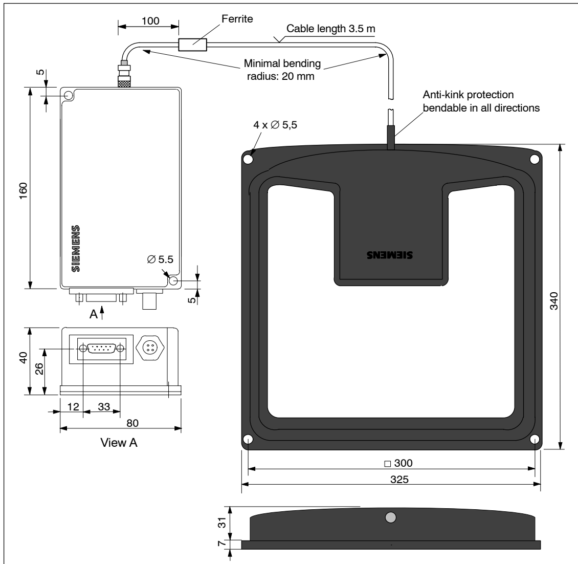
Figure 5-13 Dimensioned drawing of the SLG D11 ANT D5
