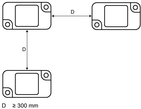
Figure 6-2 Minimum distance ANT 1
