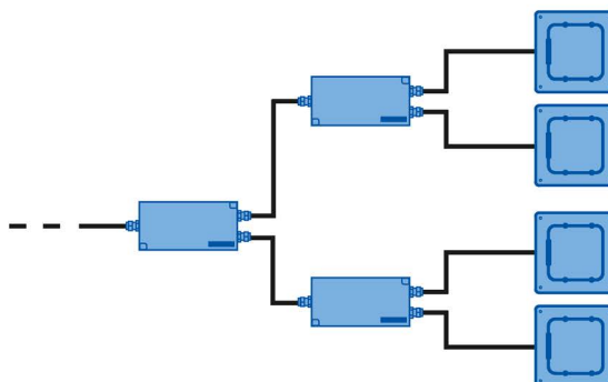
Figure 4-16 Possible configuration of RF290R with ANT D5/D6/D10
