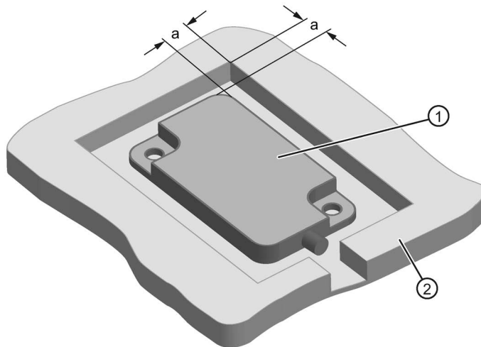
Figure 6-5 ANT 3 mounted on metal
