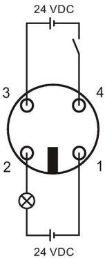
Figure 5-19 Pin assignment of the power supply connector
