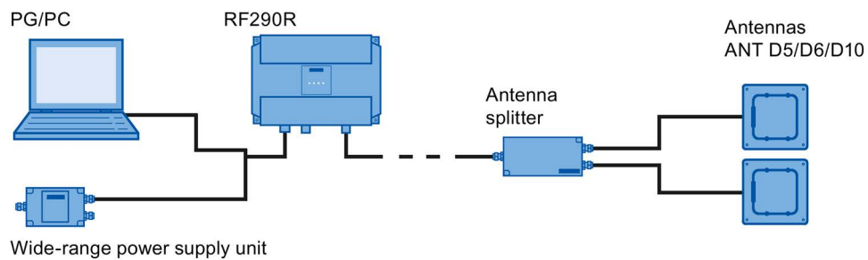
Configuration with 2 antennas (gate)
