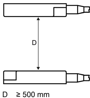
Figure 6-3 Face-to-face minimum distance ANT 1
