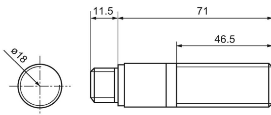
Figure 5-3 RF210R dimension drawing
