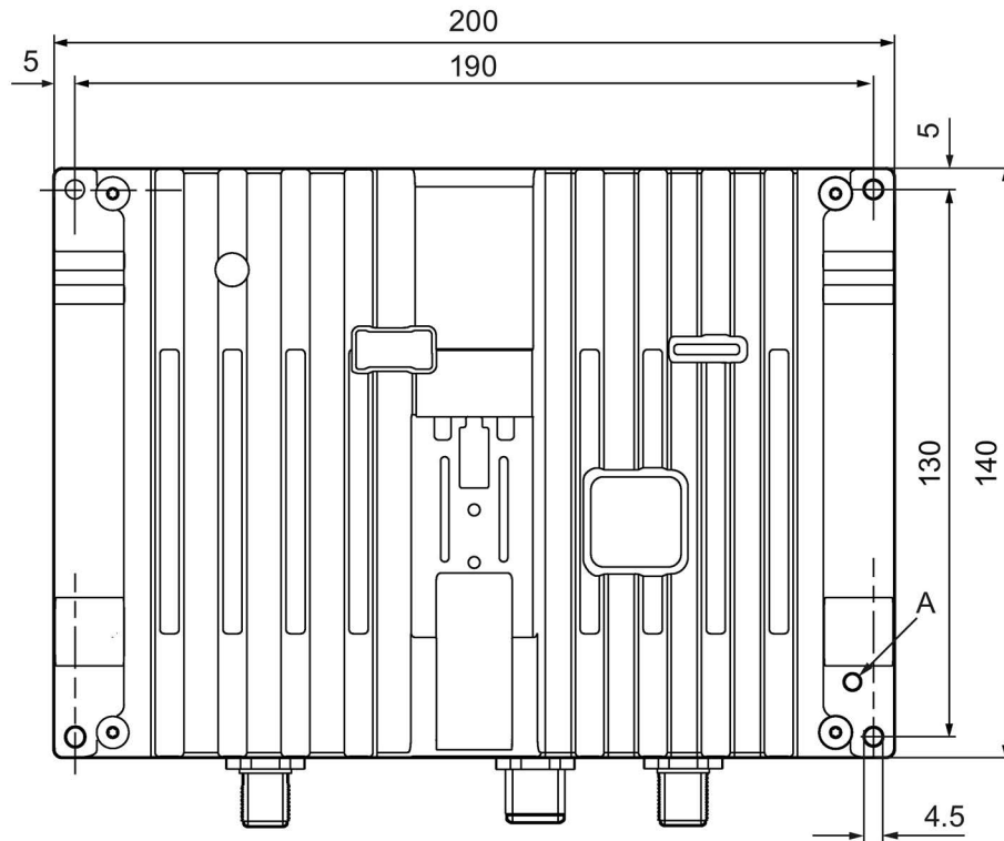
Figure 5-20 Drilling pattern for the RF290R (dimensions in mm)
