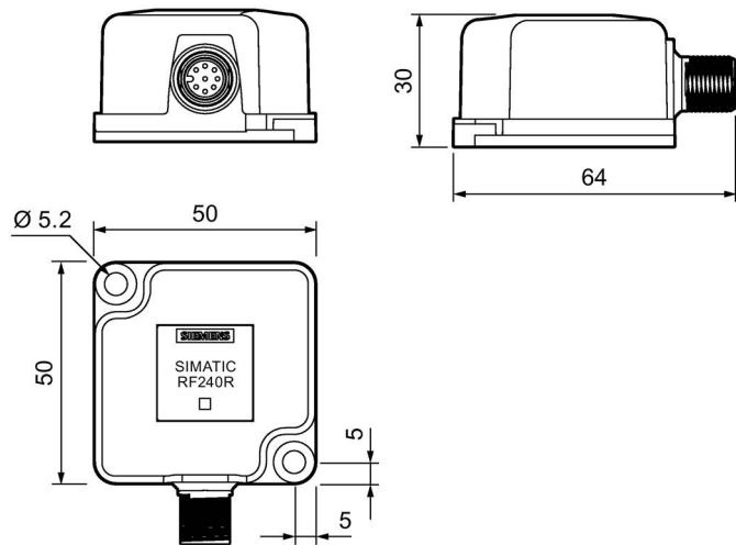
Figure 5-11 Dimension drawing RF240R Dimensions in mm
