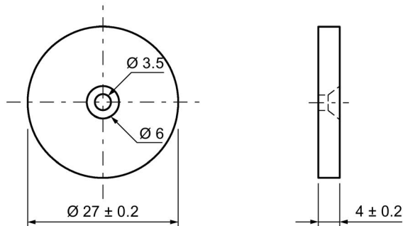
Figure 7-28 Dimension drawing of MDS D324
