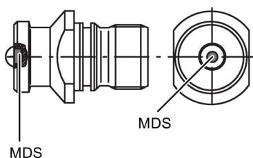
Figure 7-65 Installation example of MDS D521 in a stud bolt
