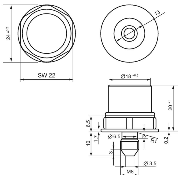
Figure 7-57 Dimension drawing of MDS D428
