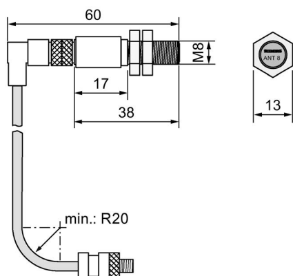
Figure 6-14 Dimension drawing ANT 8 (all values in mm)
