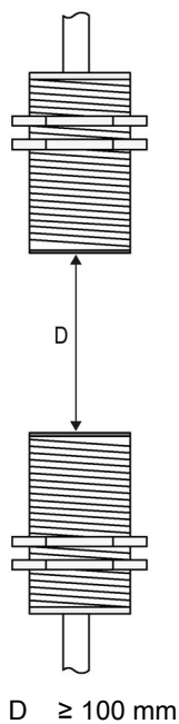
Figure 6-18 Face-to-face distance between two ANT 12s
