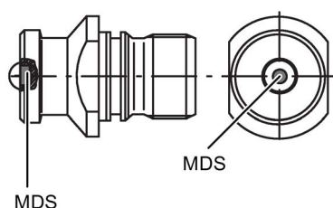
Figure 7-40 Installation example of MDS D421 in a stud bolt
