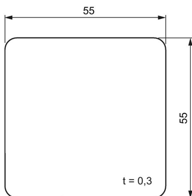
Figure 7-25 Dimension drawing of MDS D261
