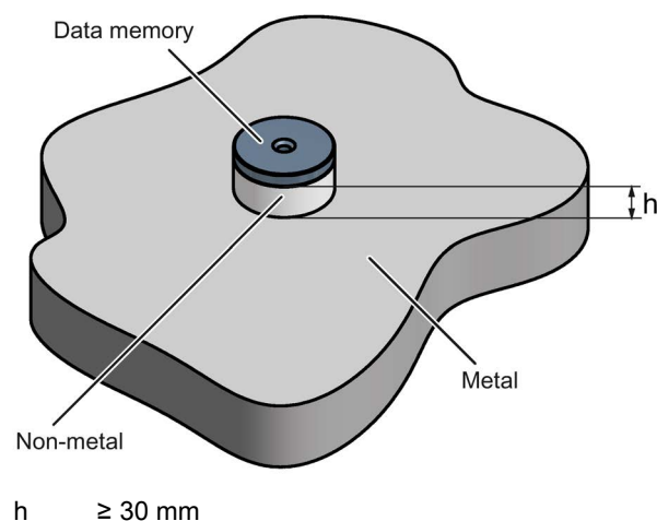
Figure 7-14 Mounting the MDS D139 on metal with spacer
