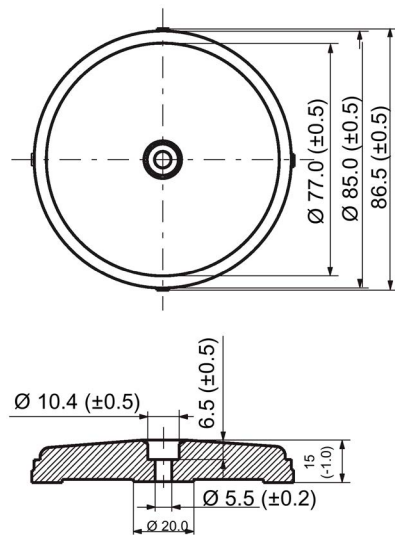
Figure 7-17 Dimensional drawing of MDS D139
