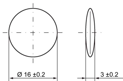
Figure 7-19 Dimensional drawing of MDS D160
