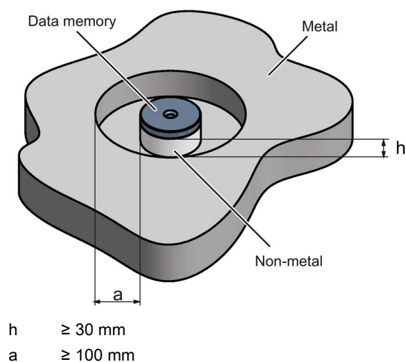
Figure 7-15 Flush-mounting of the MDS D139 in metal with spacer
