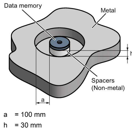
Figure 7-31 MDS D339: Mounting in metal
