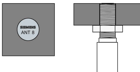
Figure 6-11 ANT 8 flush-mounted in metal
