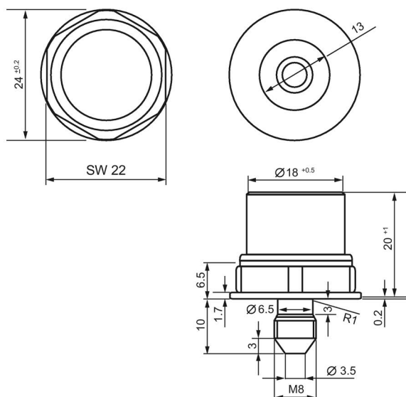
Figure 7-79 Dimensional drawing of MDS D528
