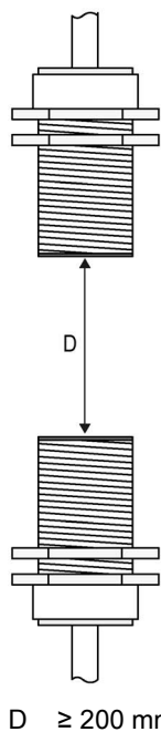
Figure 6-28 Face-to-face distance between two ANT 30s
