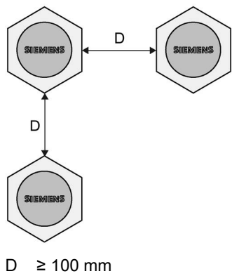
Figure 6-27 Minimum distance for ANT 30
