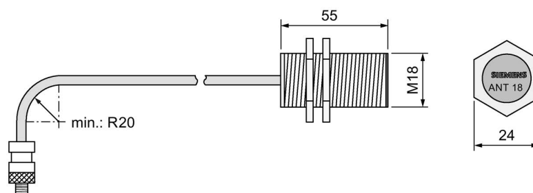
Figure 6-24 Dimension drawing ANT 18 (all values in mm)
