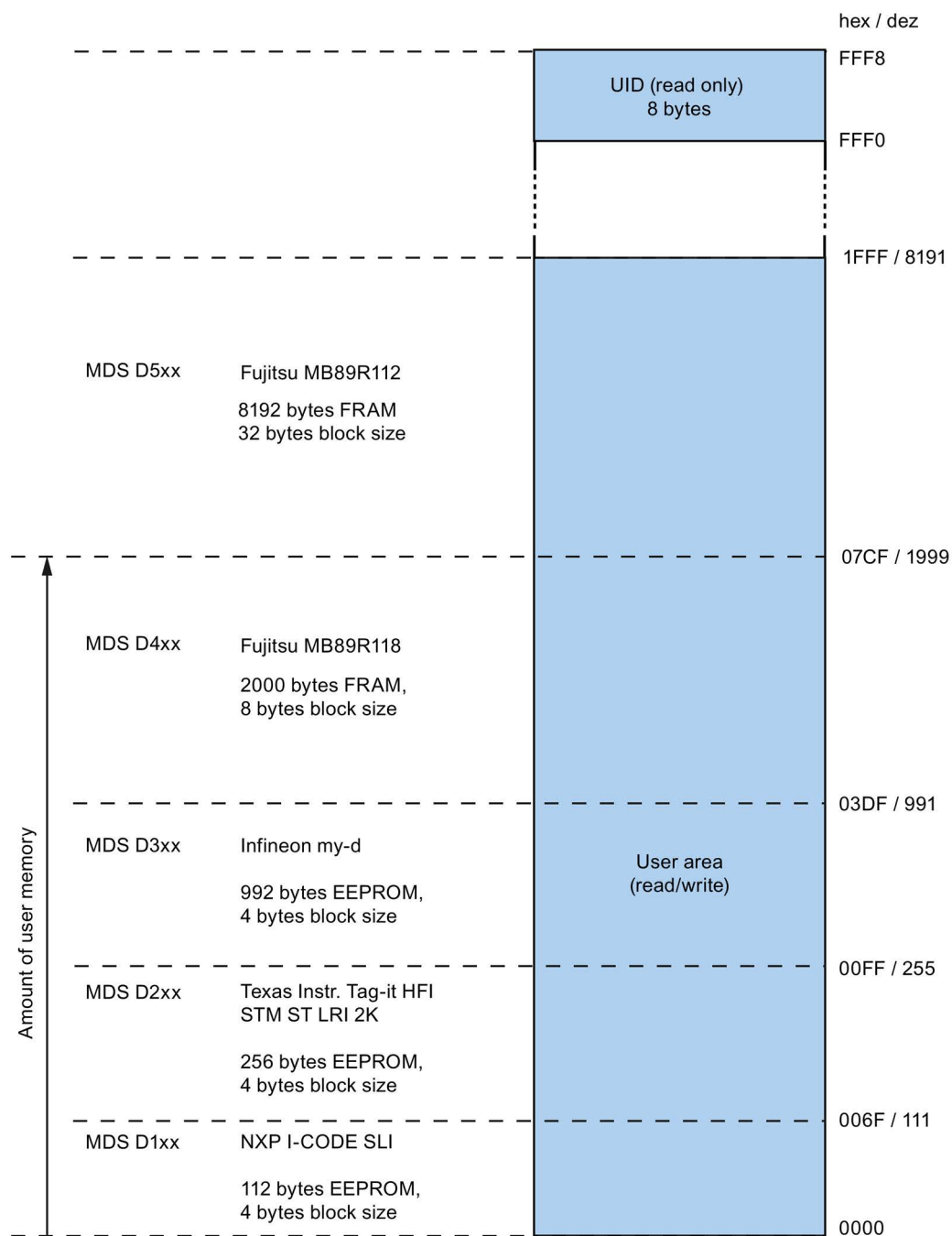
Figure 7-1 Memory configuration of ISO the transponders
