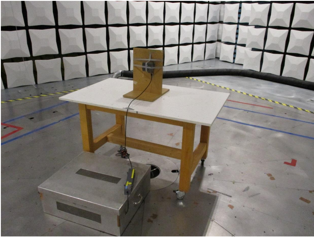
Radiated Emission Measurement (Alternate Test Site)
