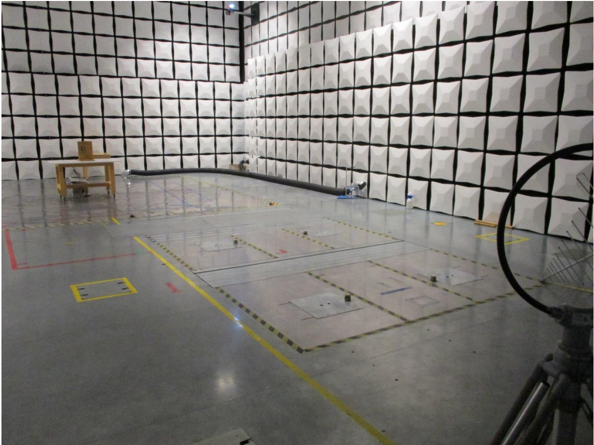
Radiated Emission Measurement 9 kHz – 30 MHz
